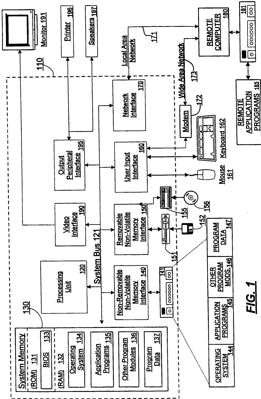
Computing Environment 100
