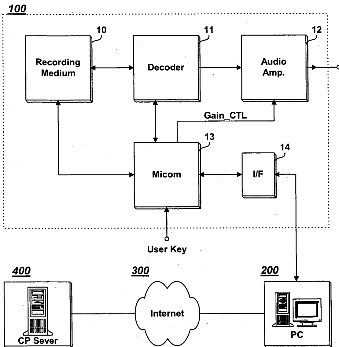
FIG. 1 (Related Art)
