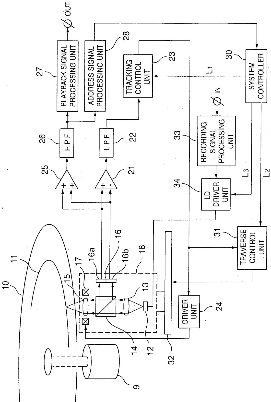
FIG.6 PRIOR ART
