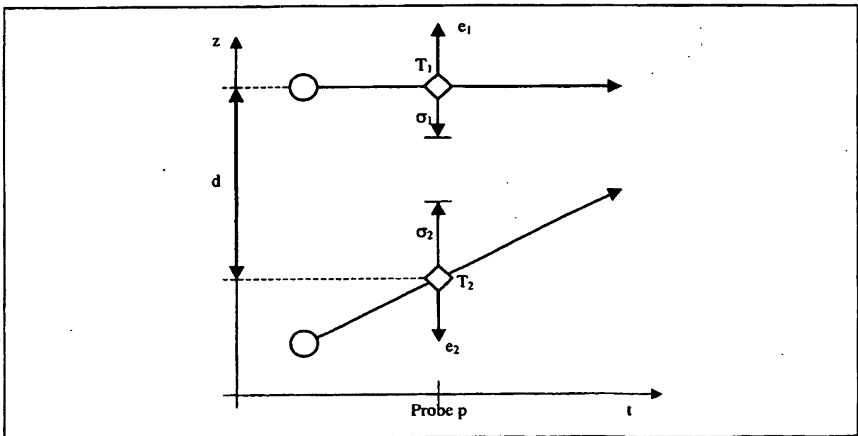
Vertical Predicted Tracks with Error Vectors and Variances of STCA
