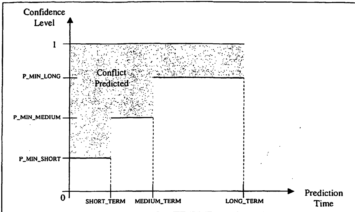
Piecewise Constant Function for Minimum Probability
