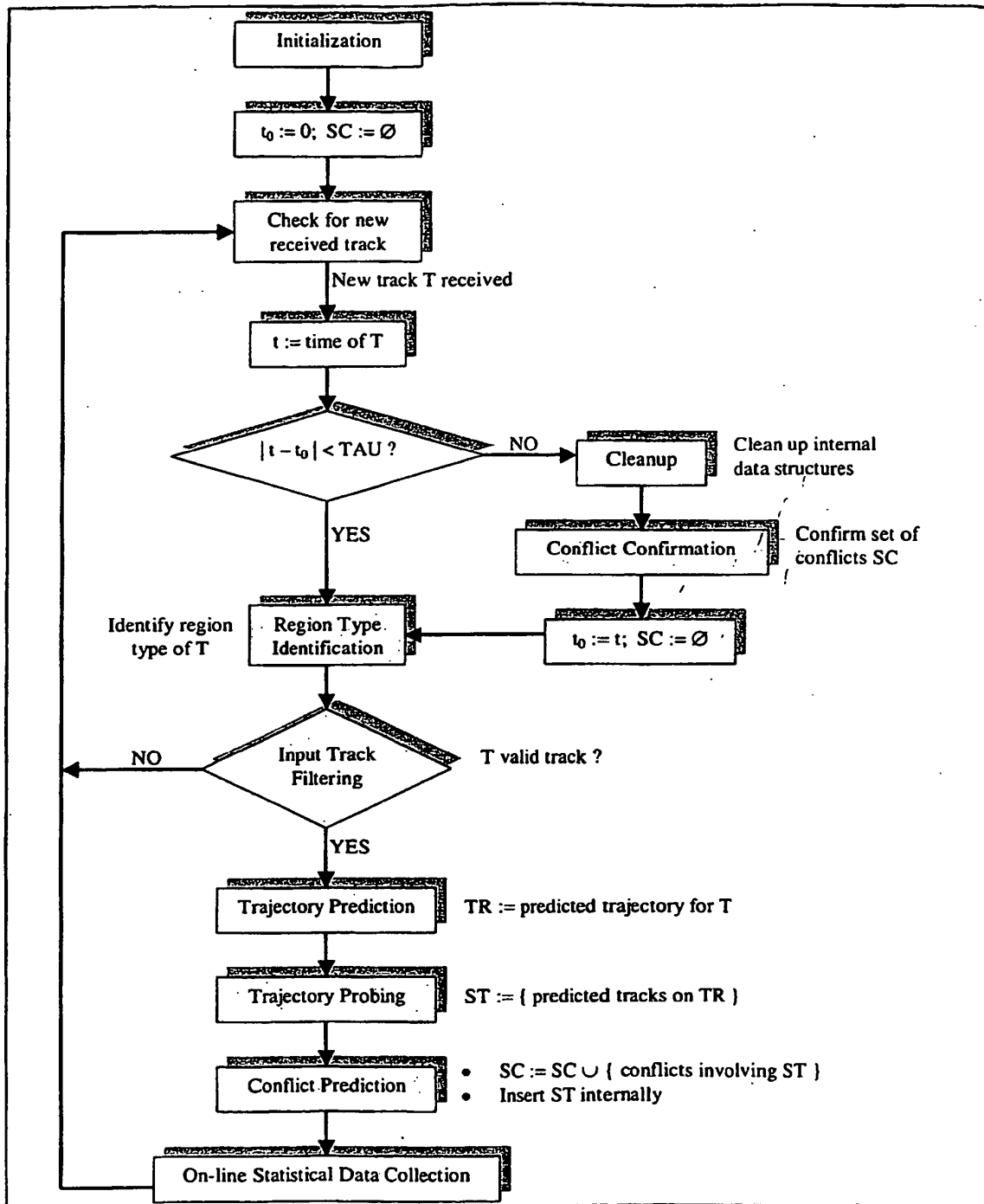
Generic Safety Net State Diagram
