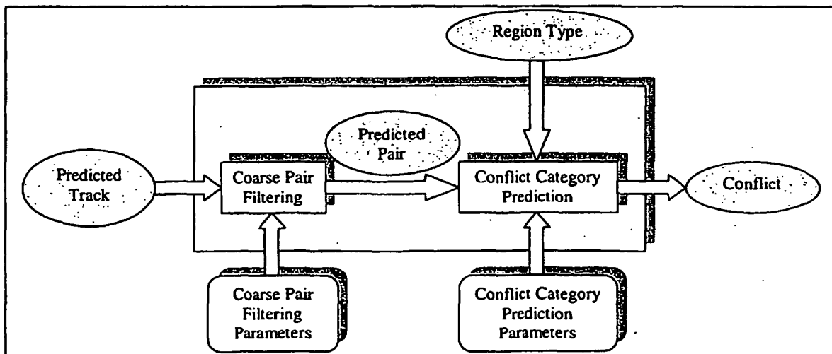
Data Flow Diagram of the Conflict Prediction Module of STCA
