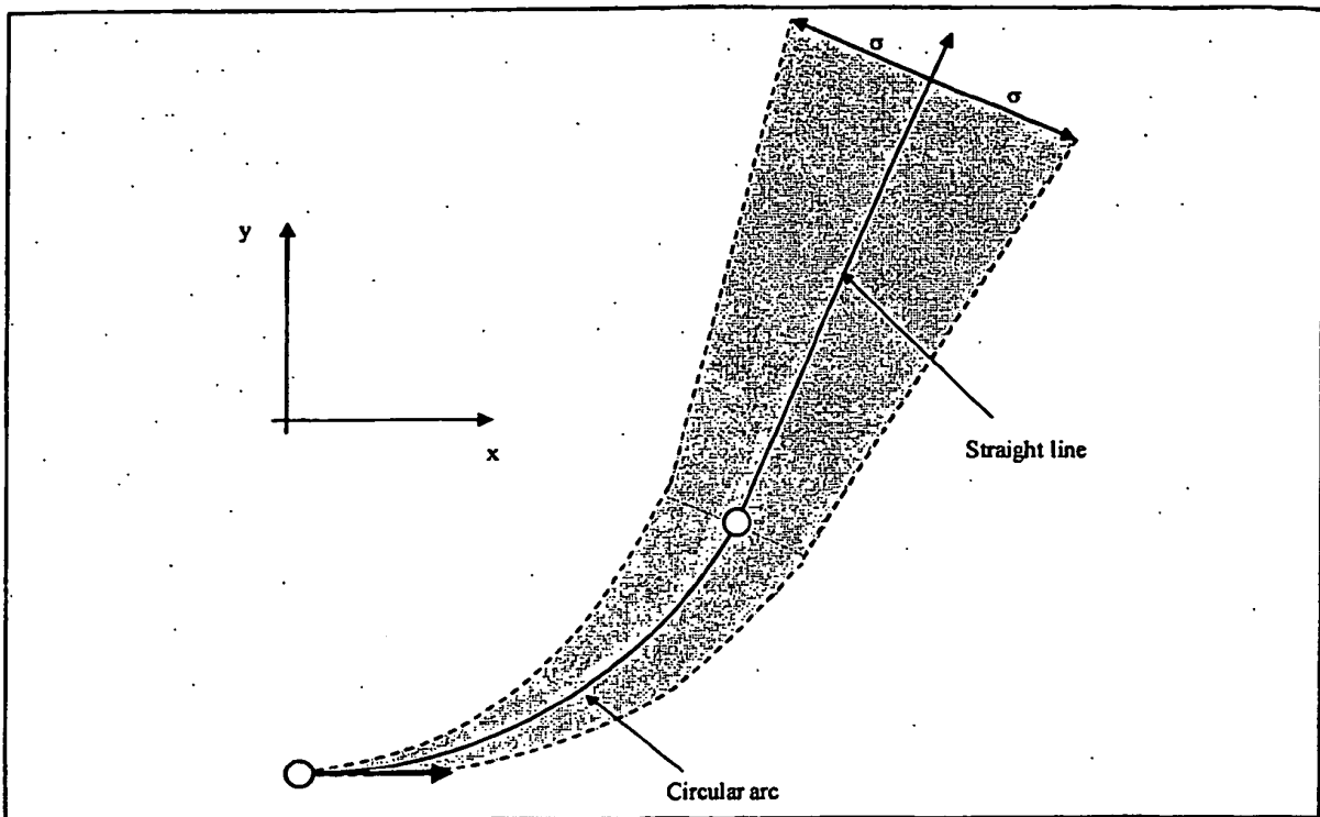
Mean Lateral Trajectory and Error Variance
