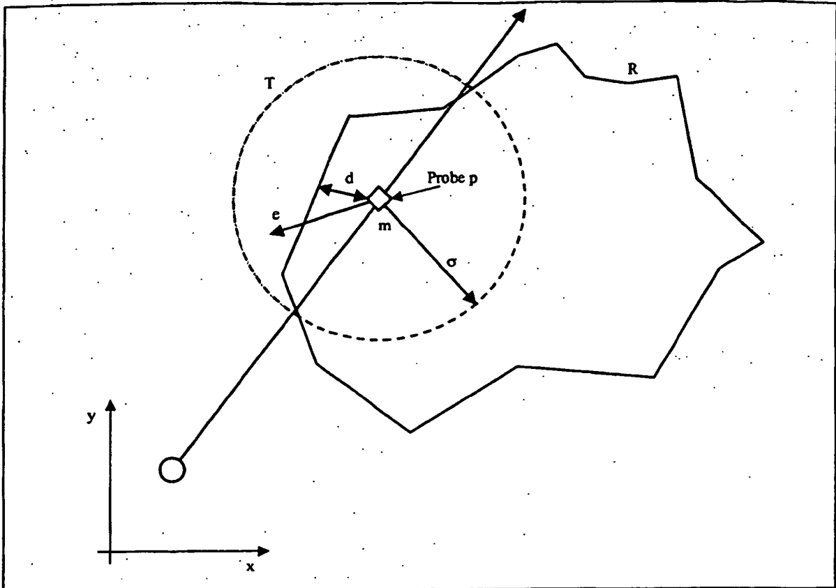
Lateral Predicted Track and Region of MSAW
