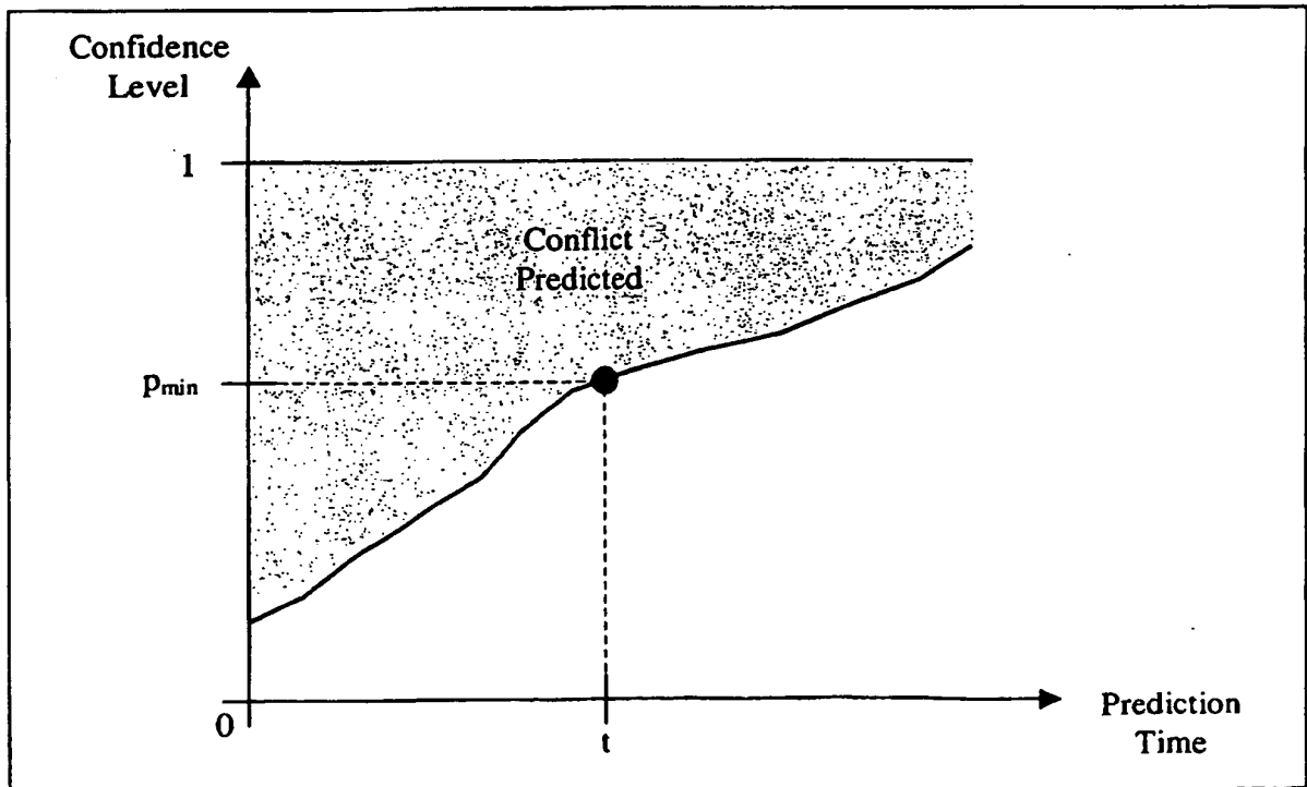
Minimum Probability as a Function of Conflict Urgency
