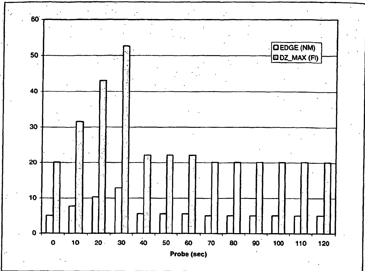
Optimal Coarse Proximity Filter Parameters for Each Probe of an example of STCA
