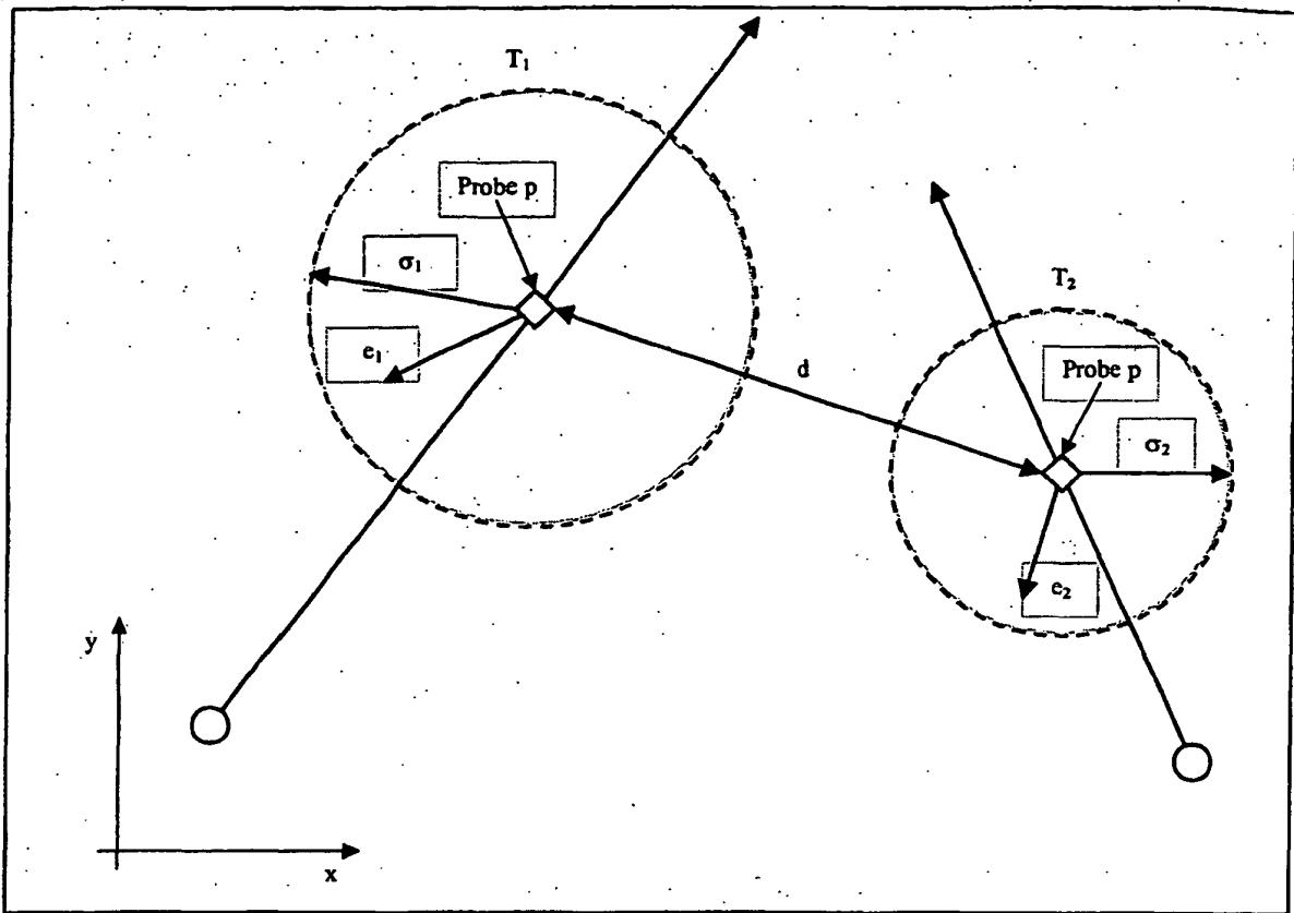
Lateral Predicted Tracks with Error Vectors and Variances of STCA
