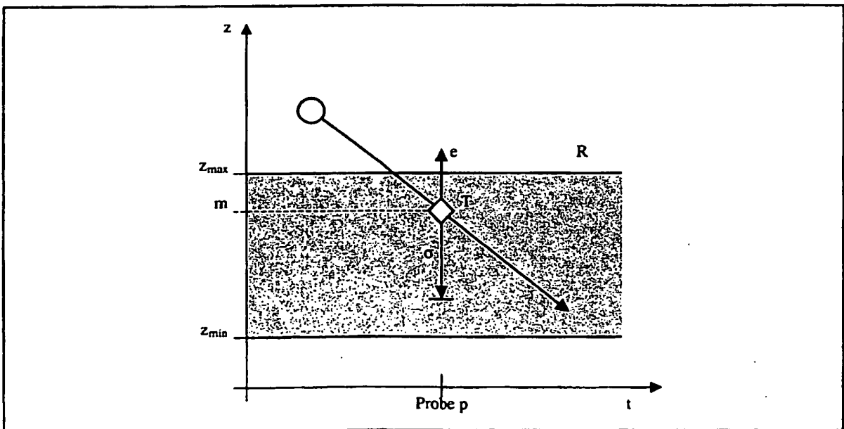
Vertical Predicted Track and Protected Region of APW
