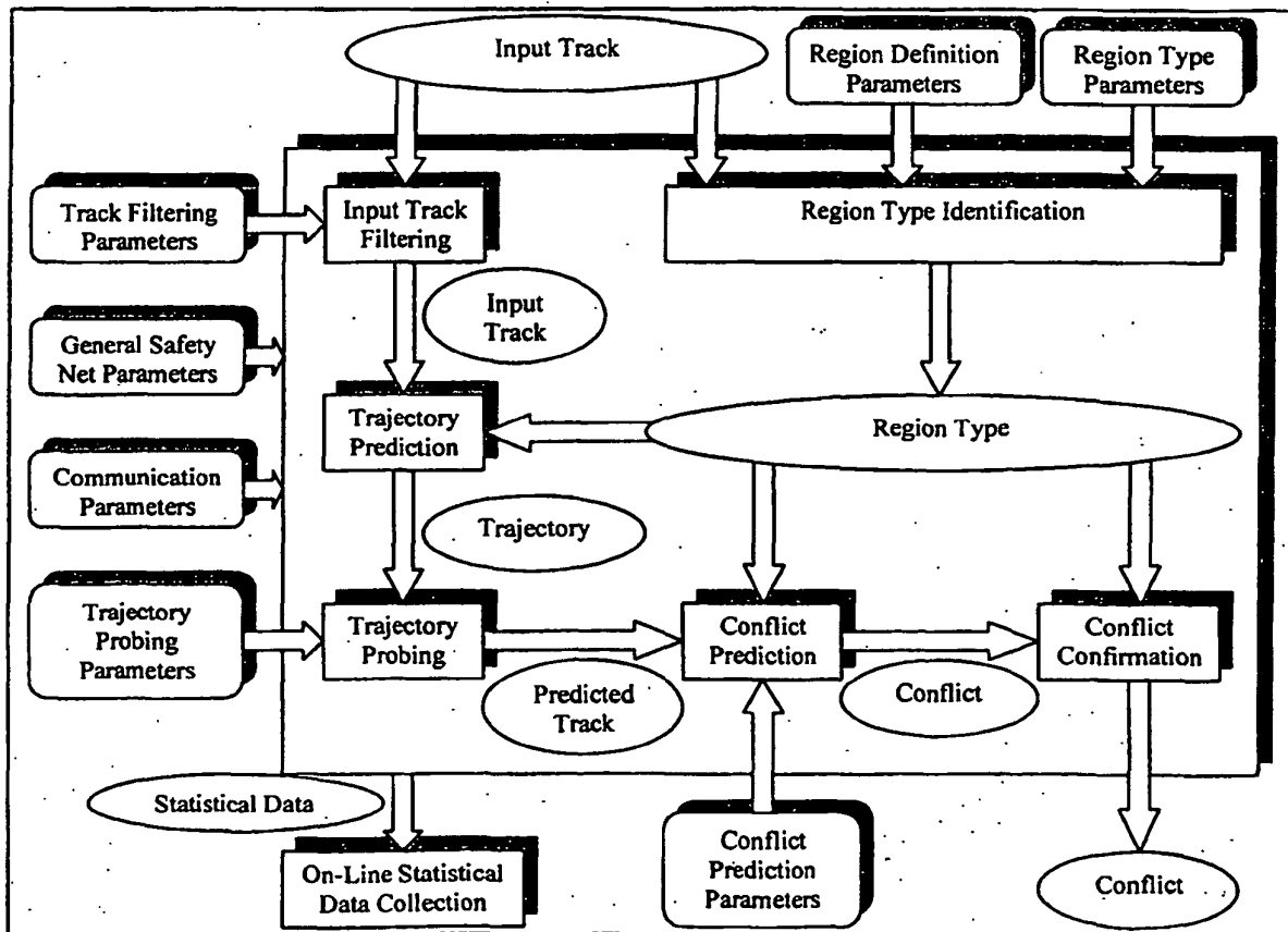
Generic Safety Net Data Flow Diagram
