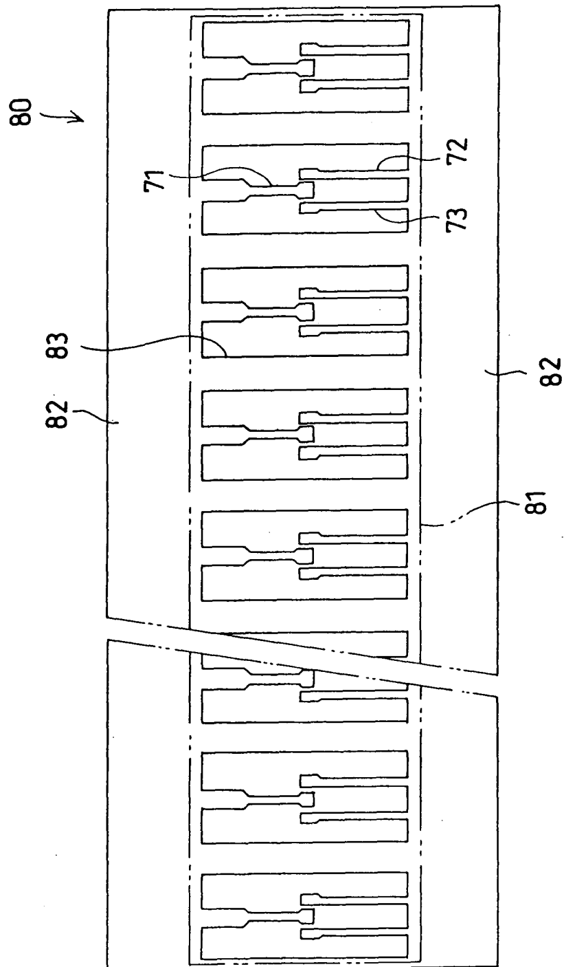
FIG. 23 PRIOR ART
