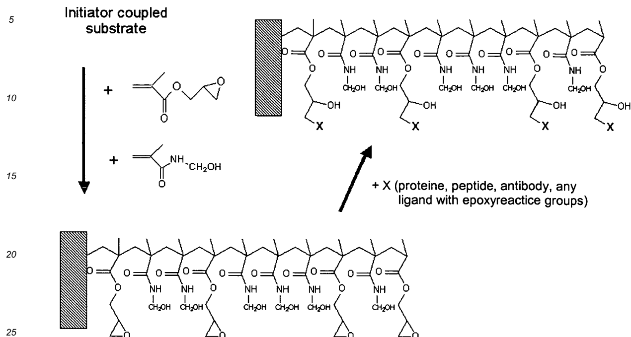
Reaction scheme 3
