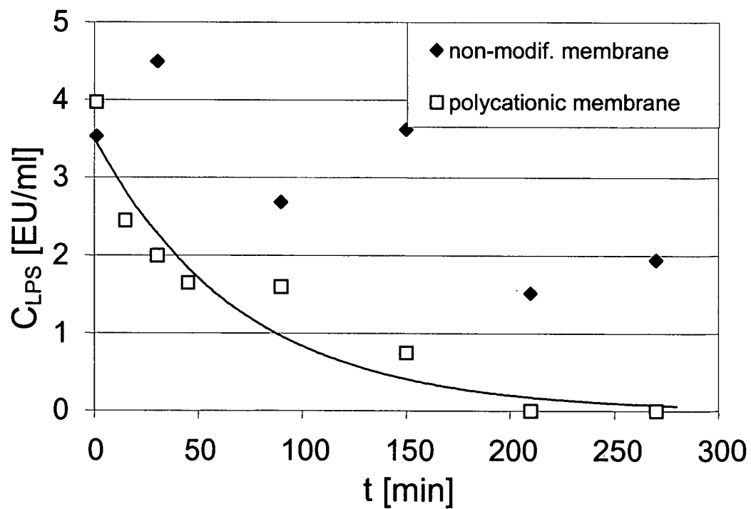
Figure 4: Endotoxin concentration in blood reservoir (example 10)
