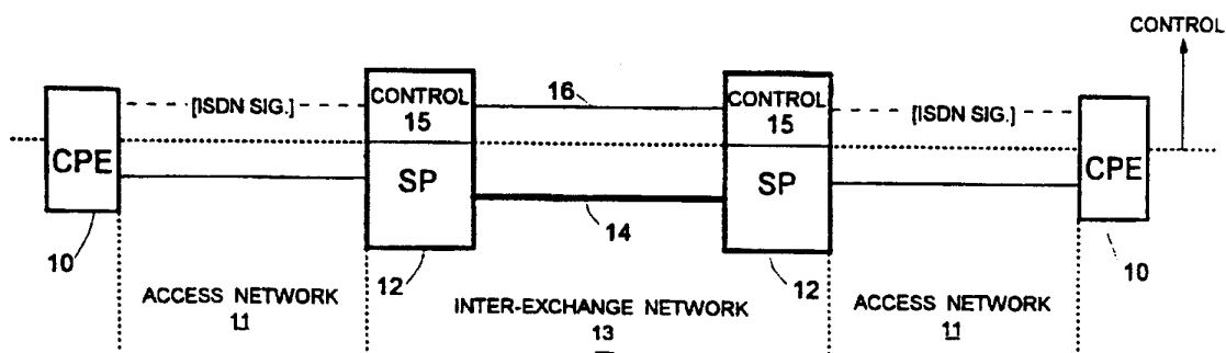
FIG. 1 (PRIOR ART)
