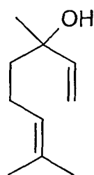
linalool
