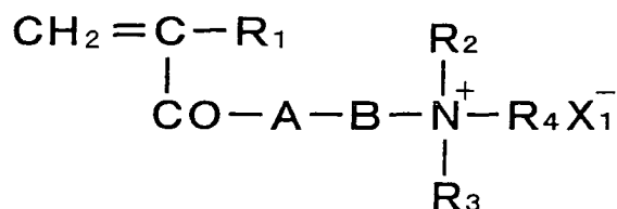
General formula (1)
