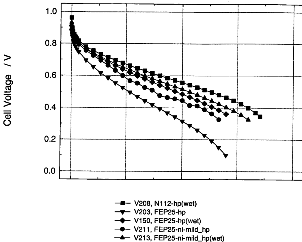
Figure 1 Typical cell polarization curves of fuel cells containing the various MEAs described in the working and comparative examples. Measurements were made after the MEAs had been conditioned subsequent to start up and attaining stable performance, typically about 100 - 150 hours. V150 (FEP25-hp(wet)) was actually measured after about 2,350 hours, but it had not degraded in performance versus the earlier measurements with this MEA.
