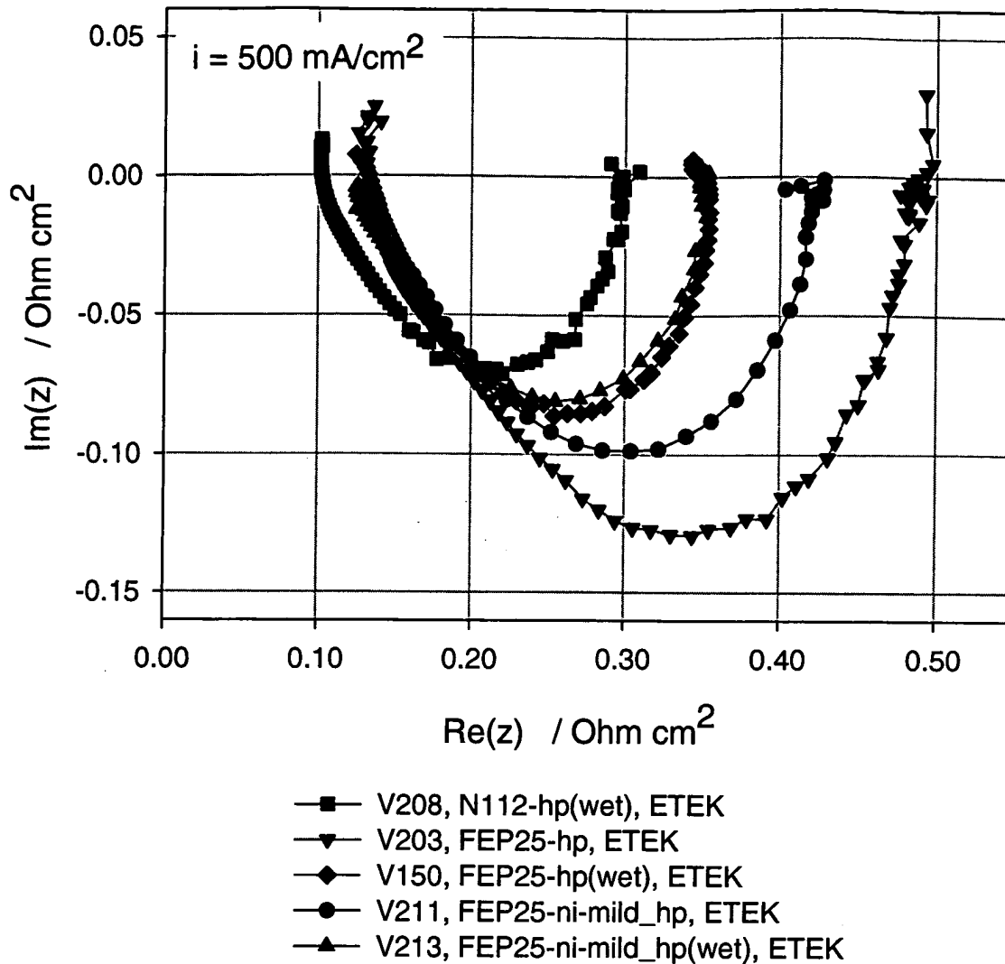
Figure 2 Typical results of electrochemical impedance spectroscopic measurements of fuel cells containing the various MEAs described in the working and comparative examples. Measurements were made after the MEAs had been conditioned subsequent to start up and attaining stable performance, typically about 100 - 150 hours. V150 (FEP25-hp(wet)) was actually measured after about 2,350 hours, but it had not degraded in performance versus the earlier measurements with this MEA.
