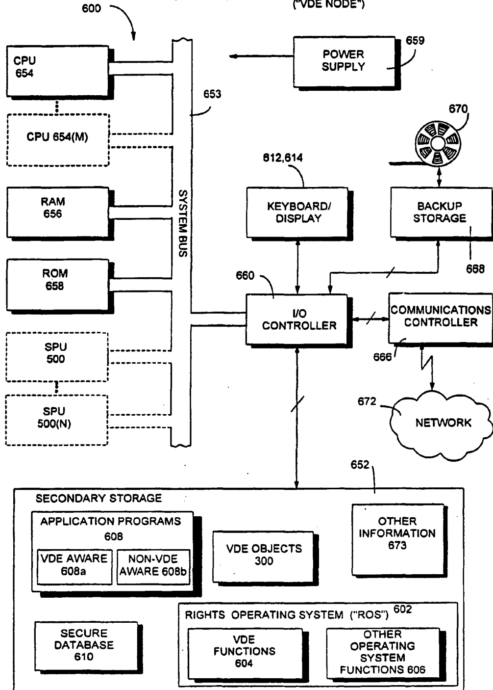
FIG. 8 ELECTRONIC APPLIANCE 600 ("VDE NODE")
