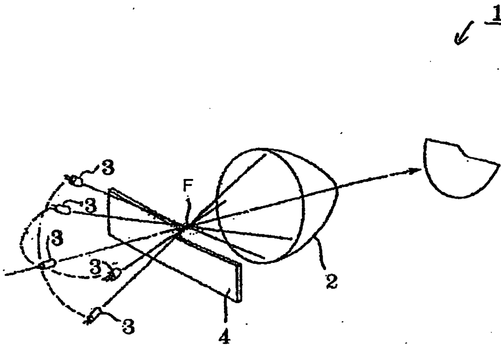
Fig. 13 Conventional Art
