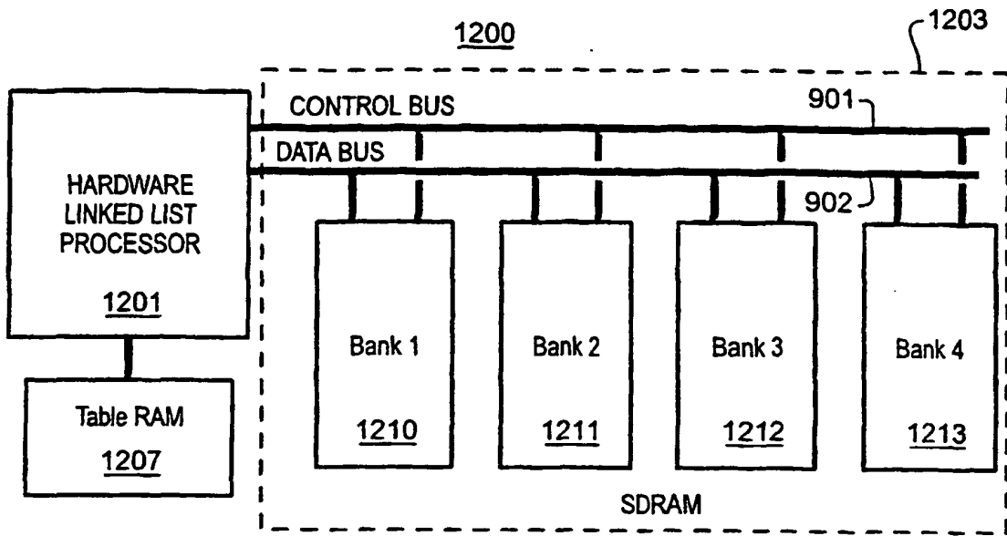
FIG. 12 PRIOR ART
