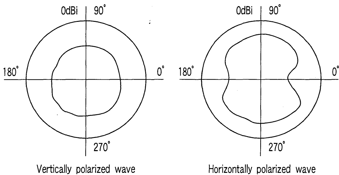
Gain characteristics of antenna A'
