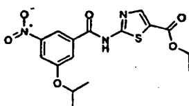
Compound (g)
