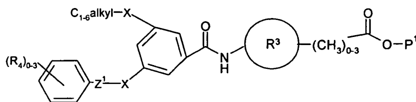
Formula (IIIc)
