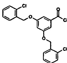
Compound (c)
