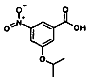
Compound (f)
