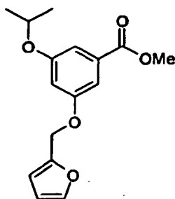
Compound (c)
