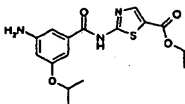
Compound (h)
