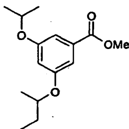
Compound (b)
