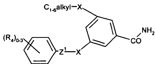
Formula (IIIf)
