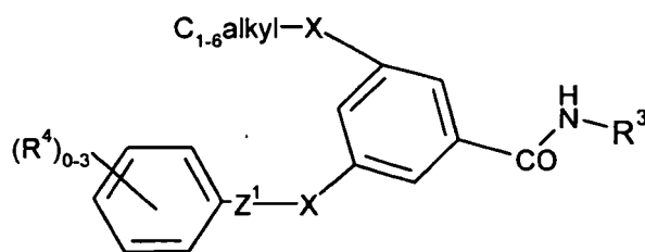
Formula (IIb)
