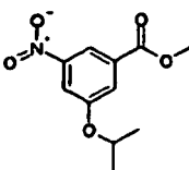
40 Compound (e)
