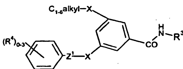
Formula (IIb)
