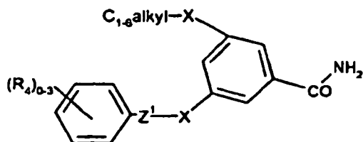
Formula (IIIf)
