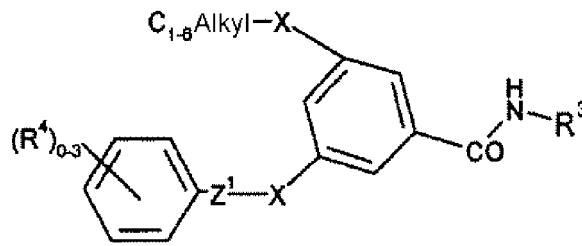
Formel (IIb)
