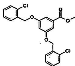
Compound (a)
