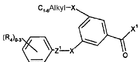
Formel (IIIa)
