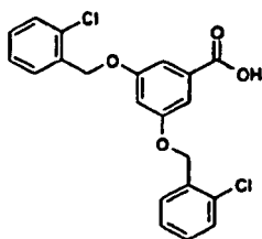
Compound (b)
