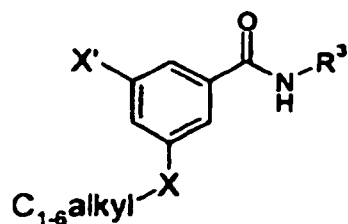
Formula (IIIe)
