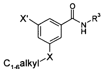
Formula (IIIe)
