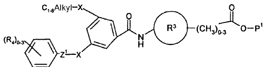
Formel (IIIc)
