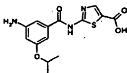
Compound (k)
