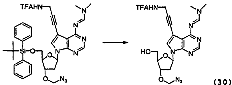
3'-O-Azidomethyl-7-deaza-4- N,N -dimethylformadin-7-[3-(2,2,2-trifluoroacetamido)-prop-1-ynyl]-2'-deoxyadenosine (30).
