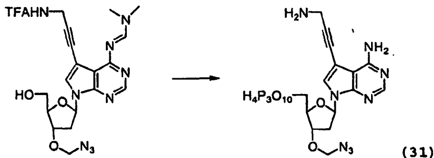
7-(3-Aminoprop-1-ynyl)-3'-O-azidomethyl -7-deaza-2'-deoxyadenosine 5'-O-nucleoside triphosphate (31).
