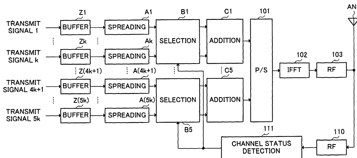
100 OFDM-CDMA TRANSMITTING APPARATUS
