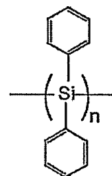
Polysilane
