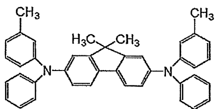
DTDPFL
