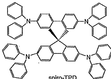
spiro-TPD
