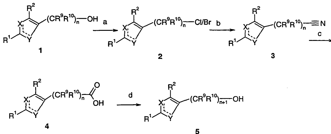
Scheme 14
