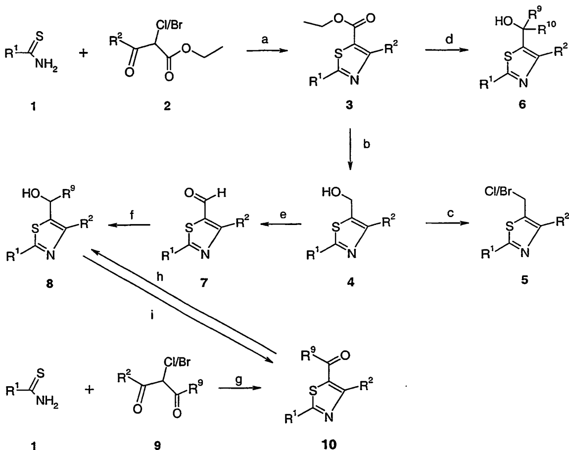
Scheme 12
