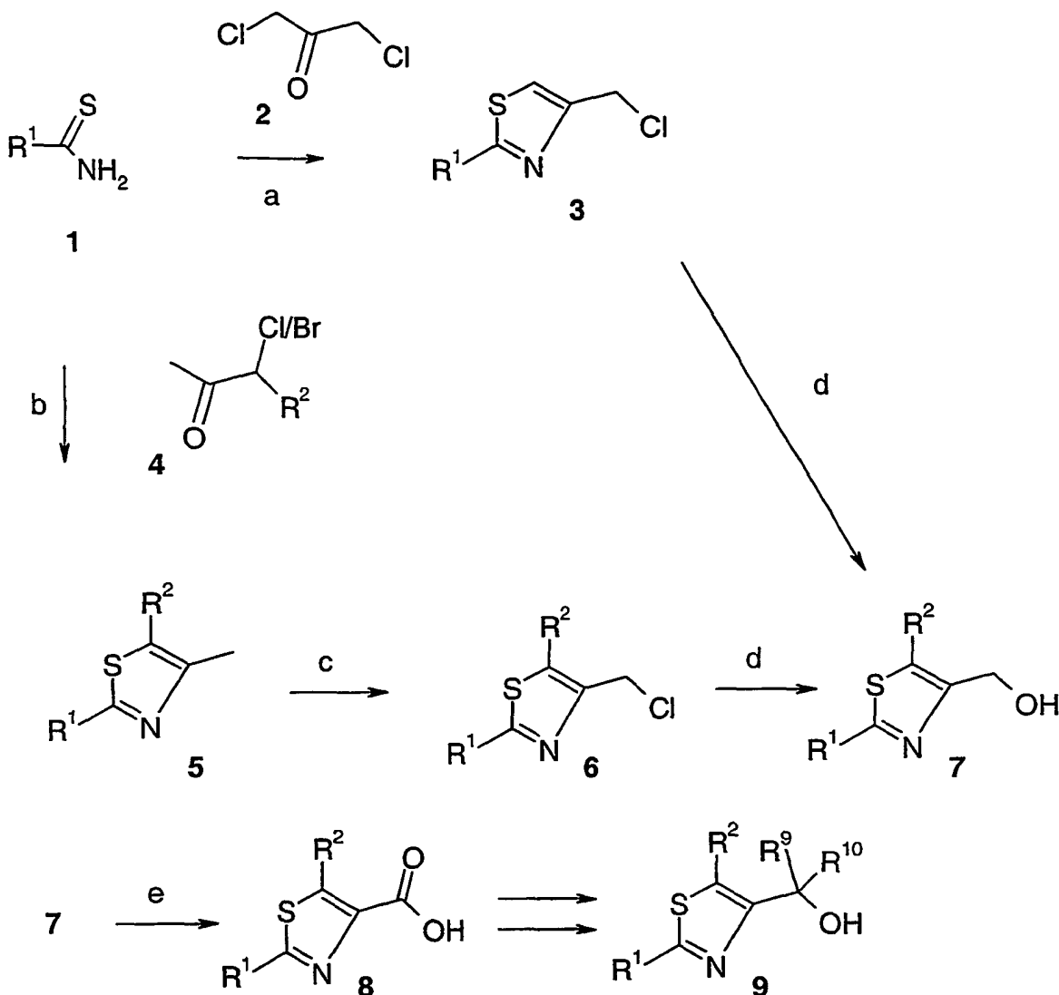
Scheme 13
