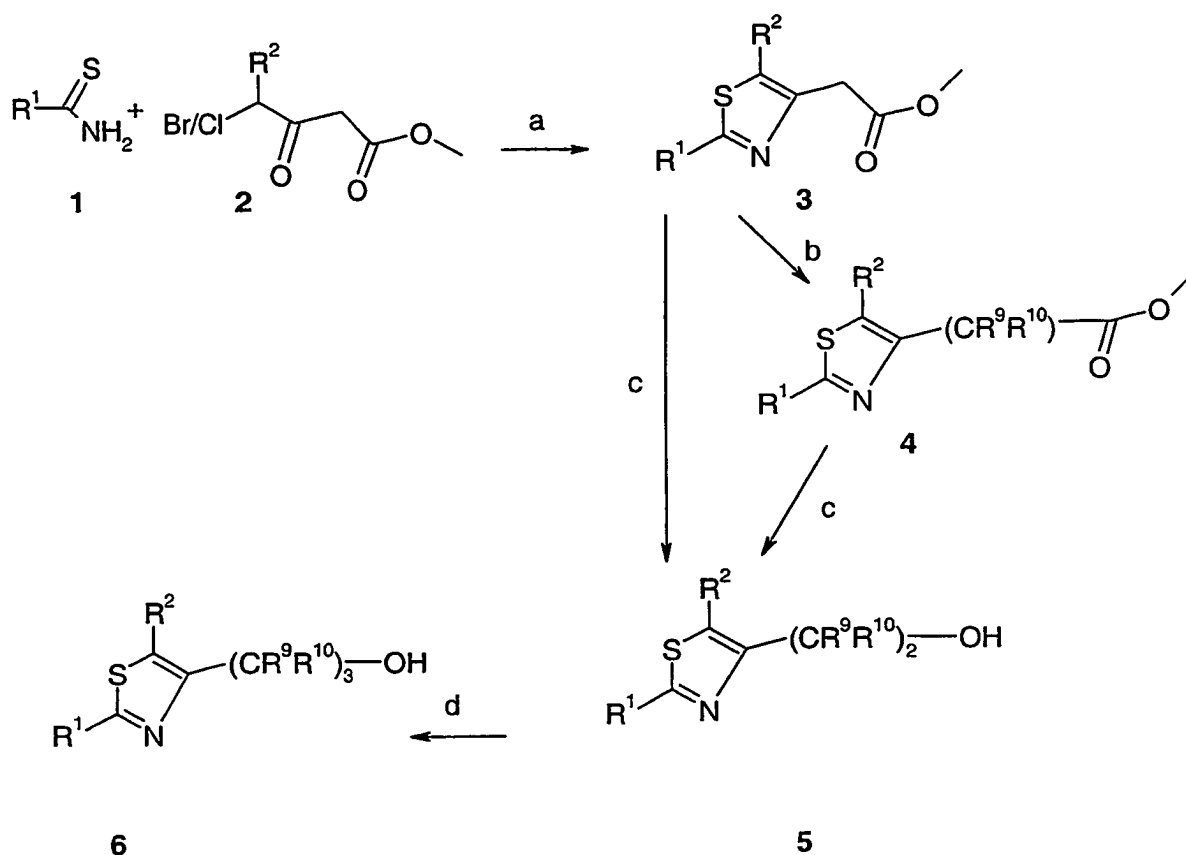
Scheme 11
