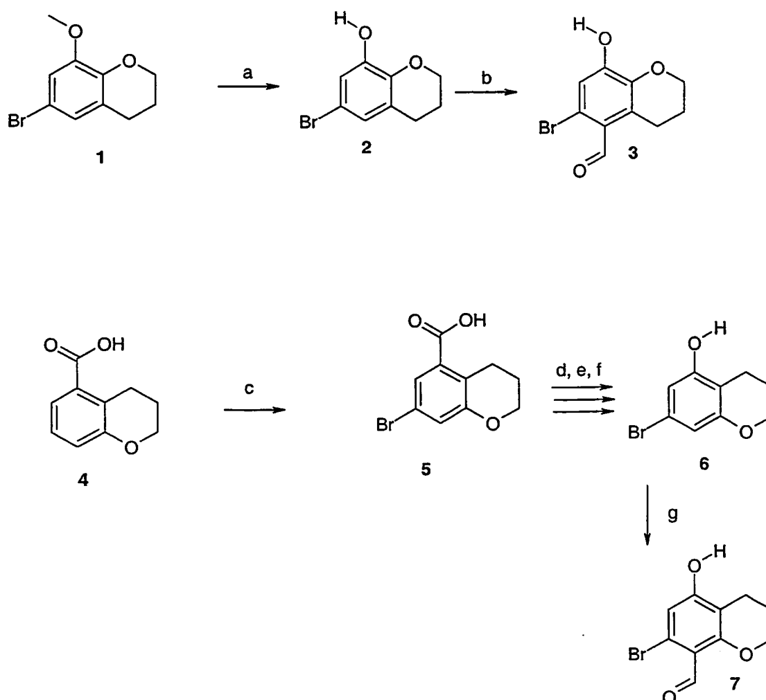
Scheme 8
