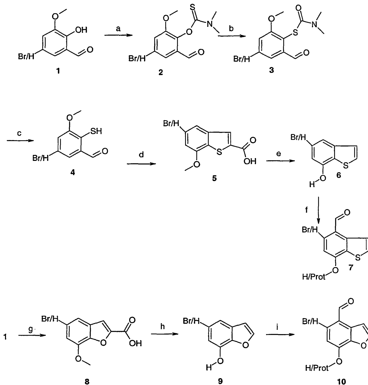
Scheme 6
