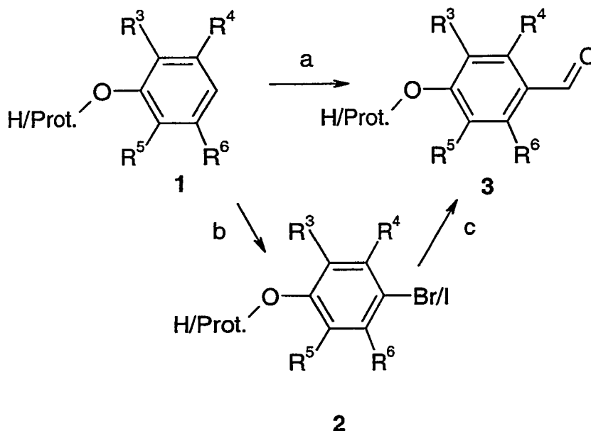
Scheme 4
