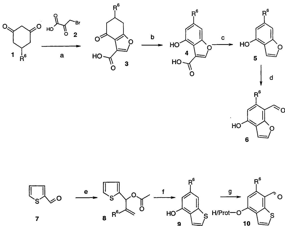
Scheme 5
