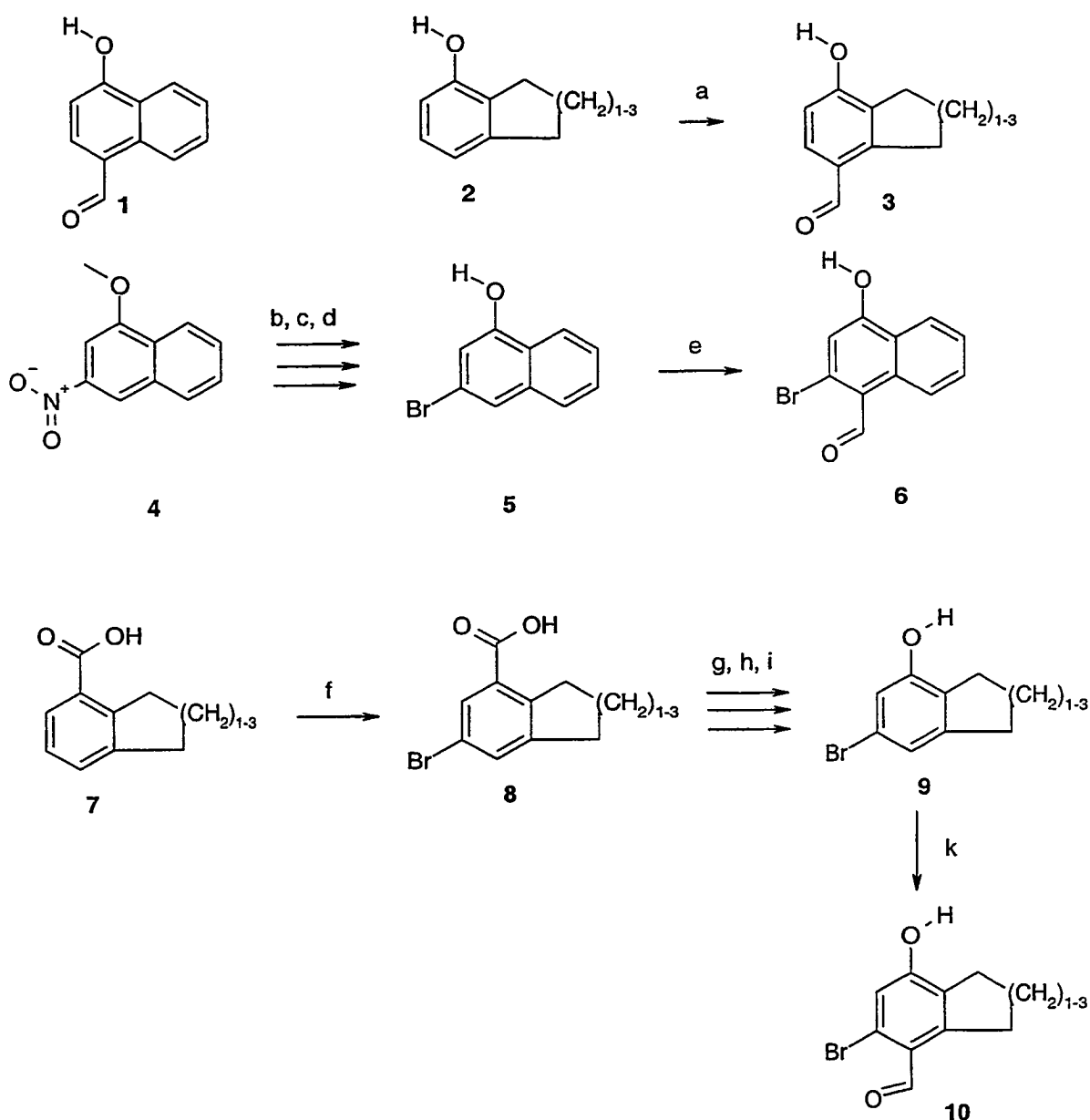
Scheme 7
