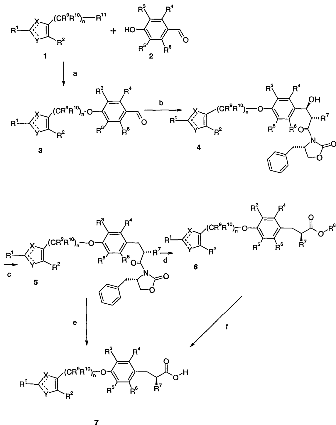
Scheme 3
