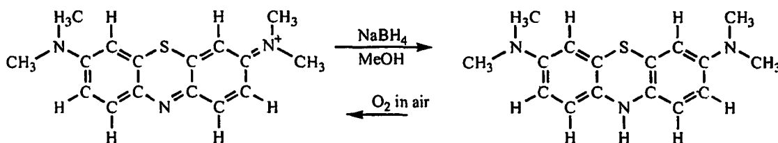
methylene blue
