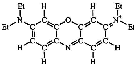
basic blue 3
