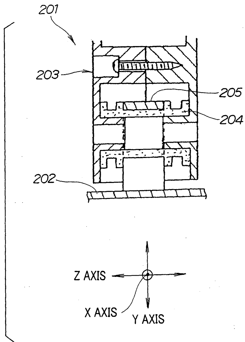
FIG. 16 (PRIOR ART)
