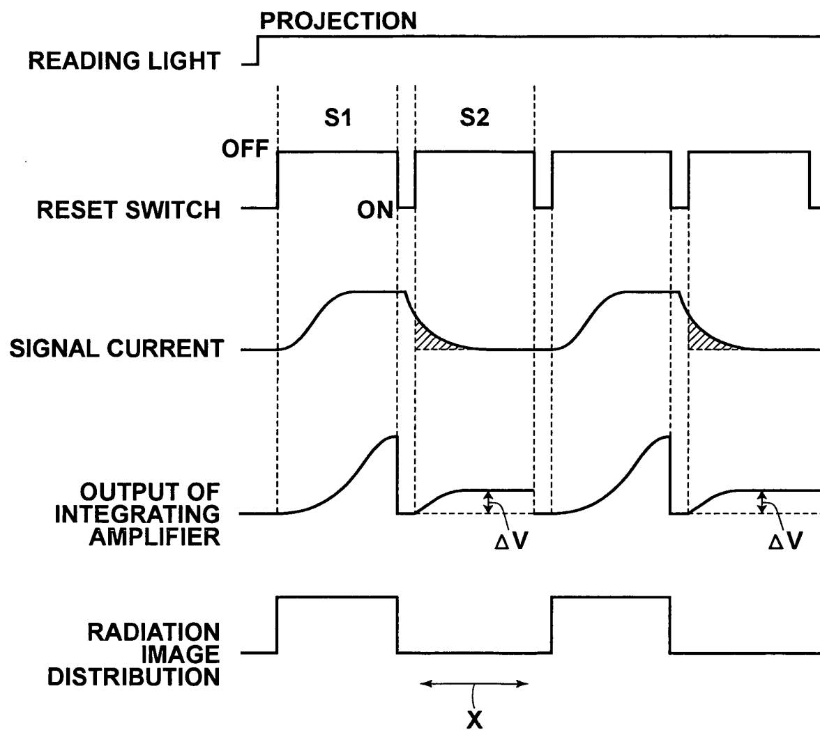
FIG.9 PRIOR ART
