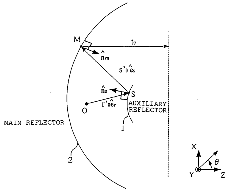
(a) XZ PLANE
