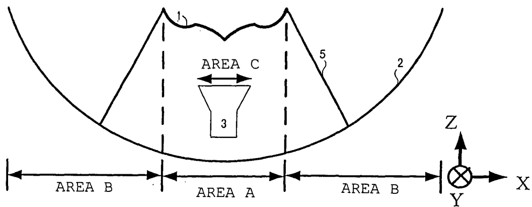
(a) REFLECTOR ON SECTION 1 (XZ PLANE)
