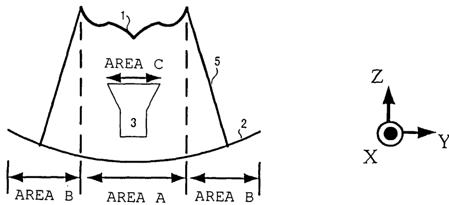
(b) REFLECTOR ON SECTION 1 (YZ PLANE)
