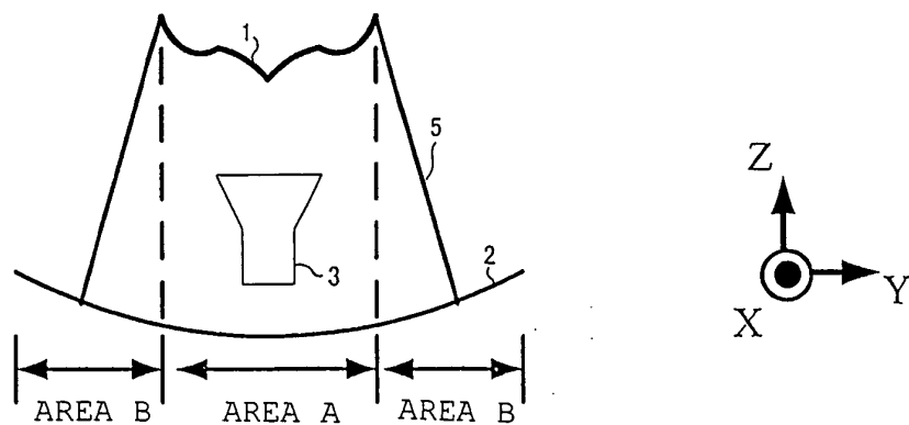
(c) REFLECTOR ON SECTION G2 (YZ PLANE)
