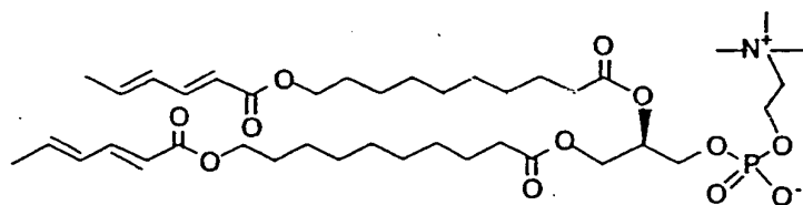
bis-SorbPC (1)
