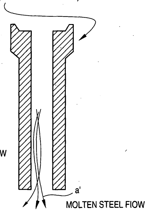
10b STRAIGHT IMMERSION NOZZLE (BOTTOM HOLE TYPE)
