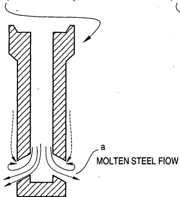
10a STRAIGHT IMMERSION NOZZLE (SIDE HOLE TYPE)
