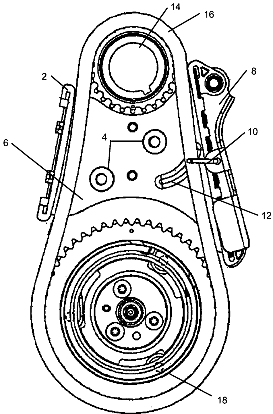
Fig. 1c PRIOR ART
