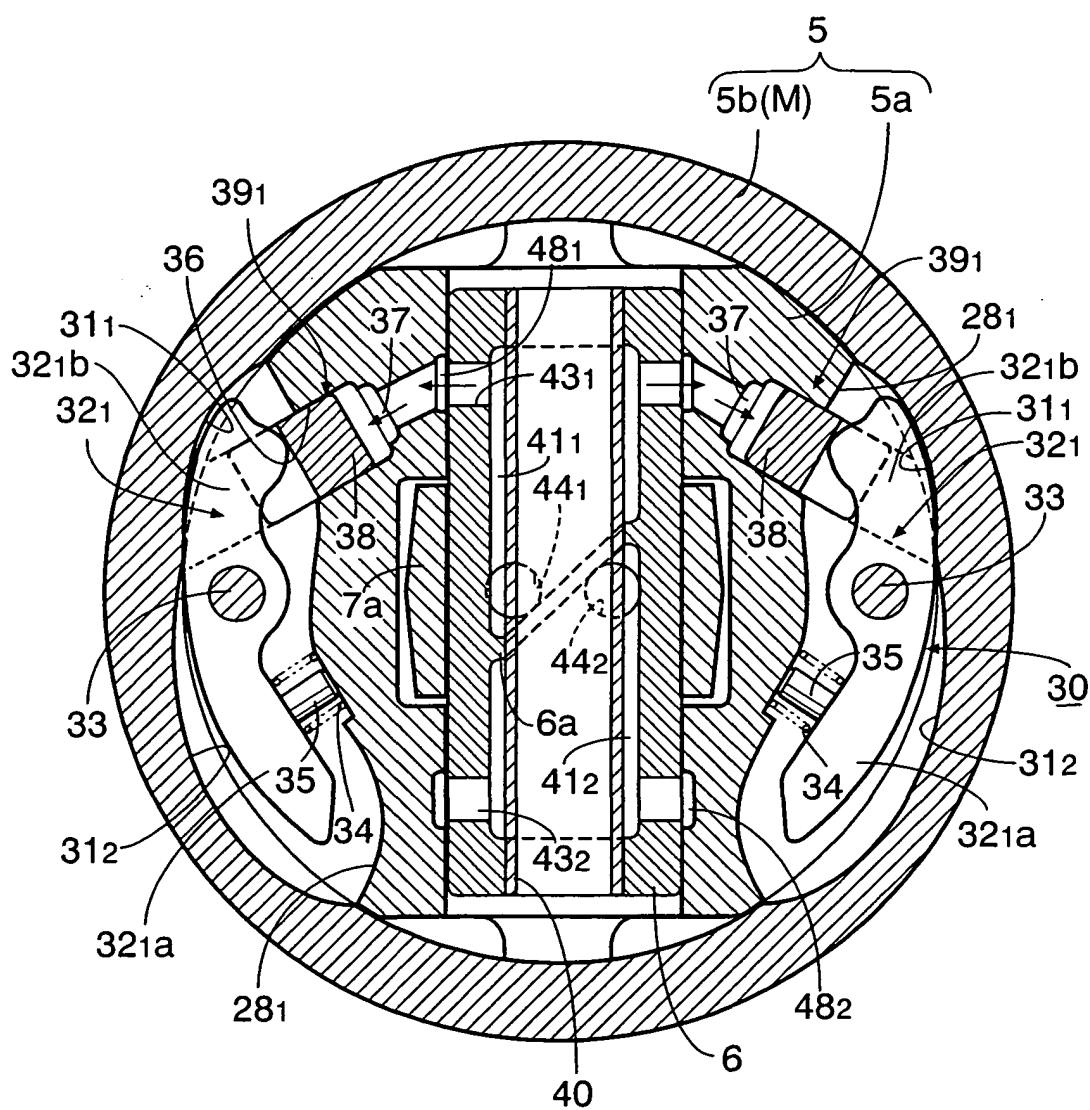
FIG.10 MEDIUM COMPRESSION RATIO STATE
