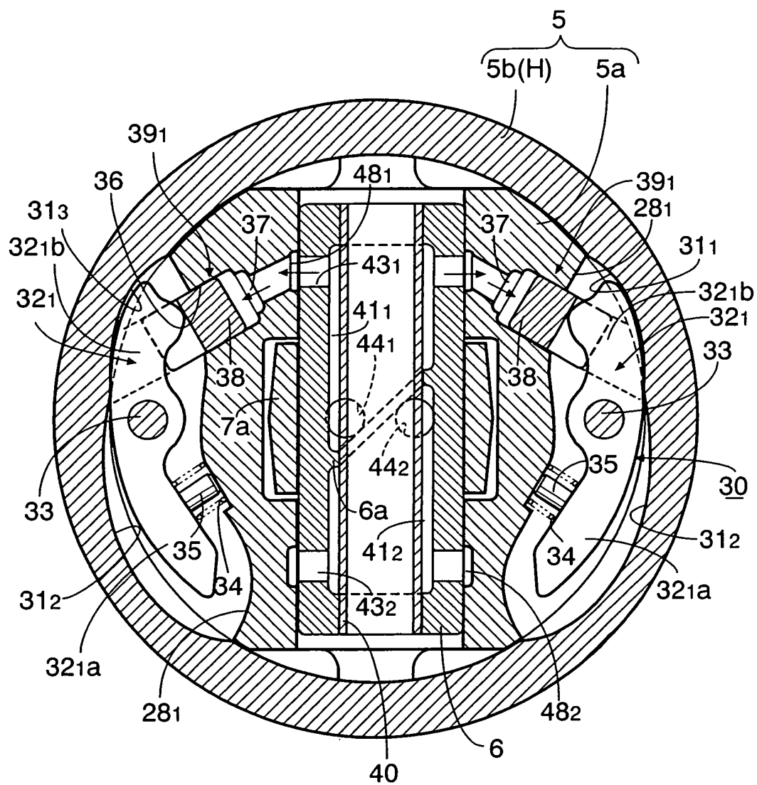
FIG.14 HIGH COMPRESSION RATIO STATE
