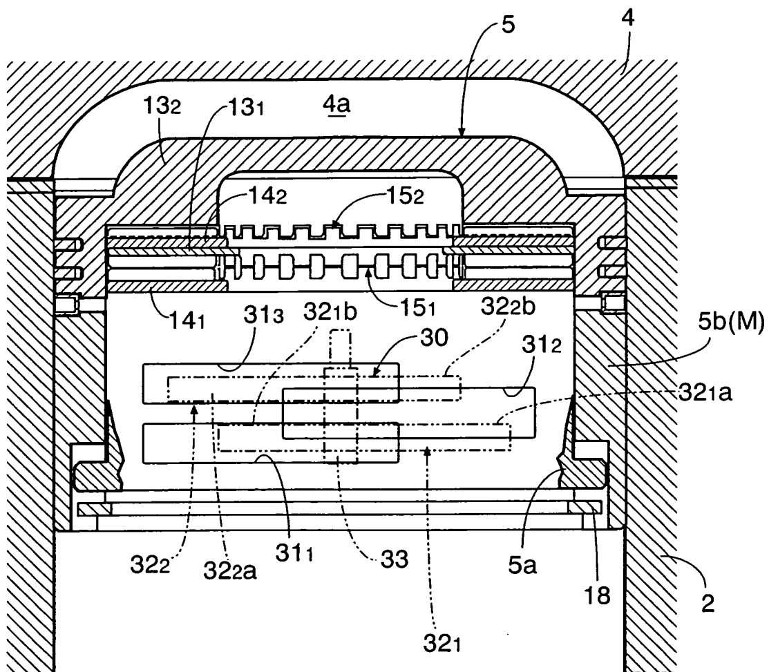
FIG.18 MEDIUM COMPRESSION RATIO STATE
