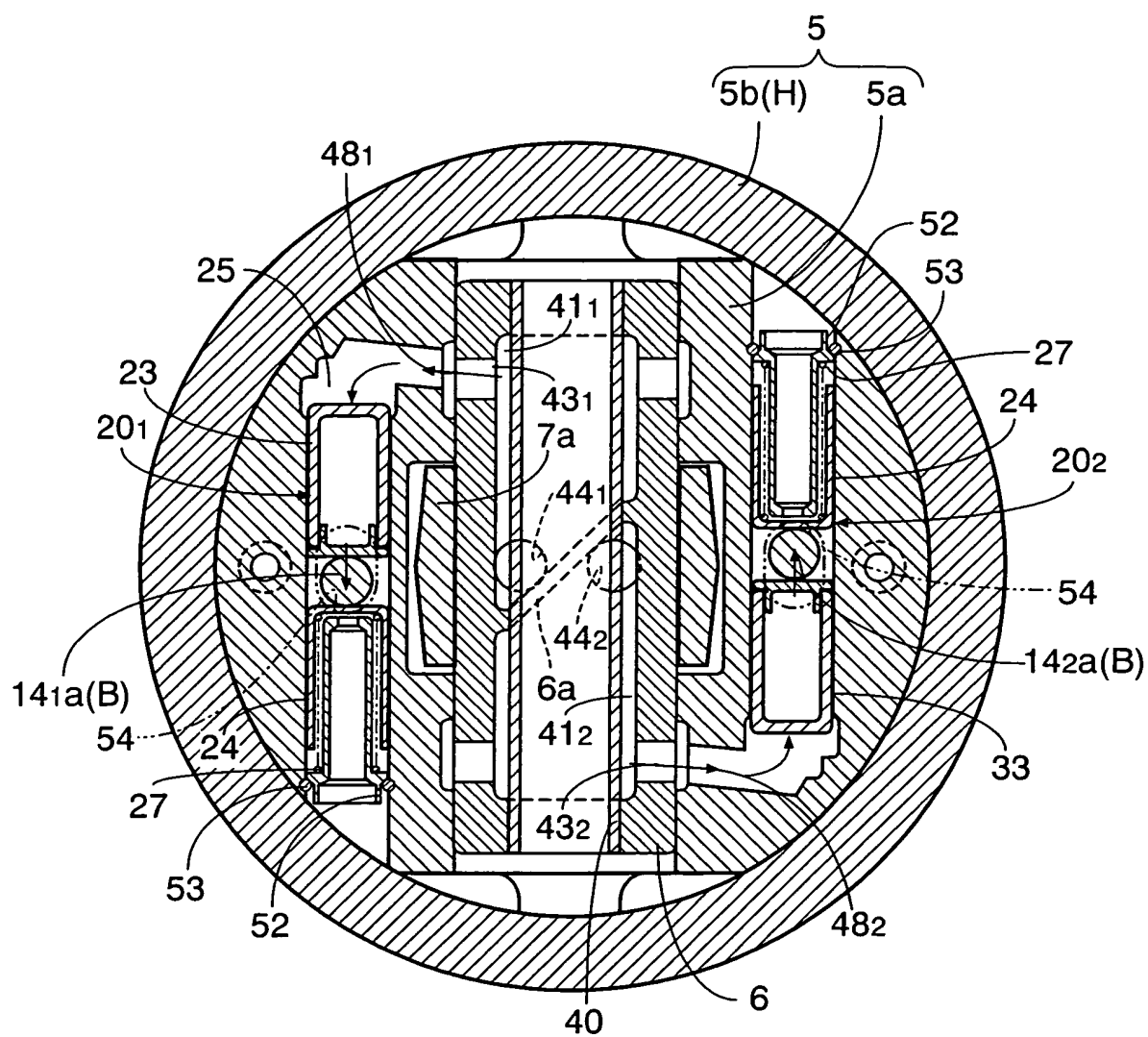
FIG.16 HIGH COMPRESSION RATIO STATE
