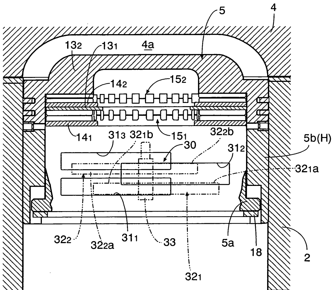
FIG.19 HIGH COMPRESSION RATIO STATE
