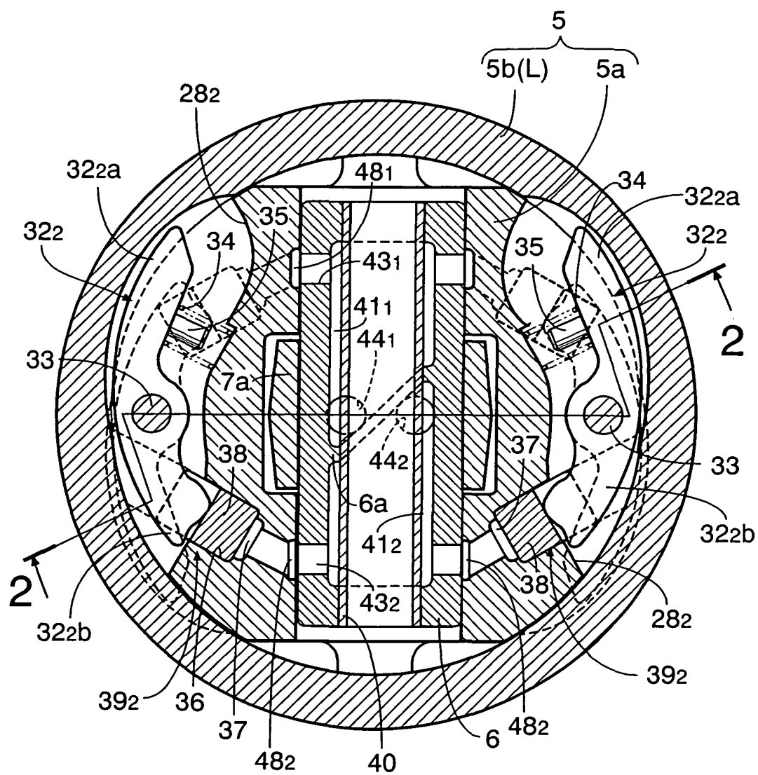
FIG.5 LOW COMPRESSION RATIO STATE
