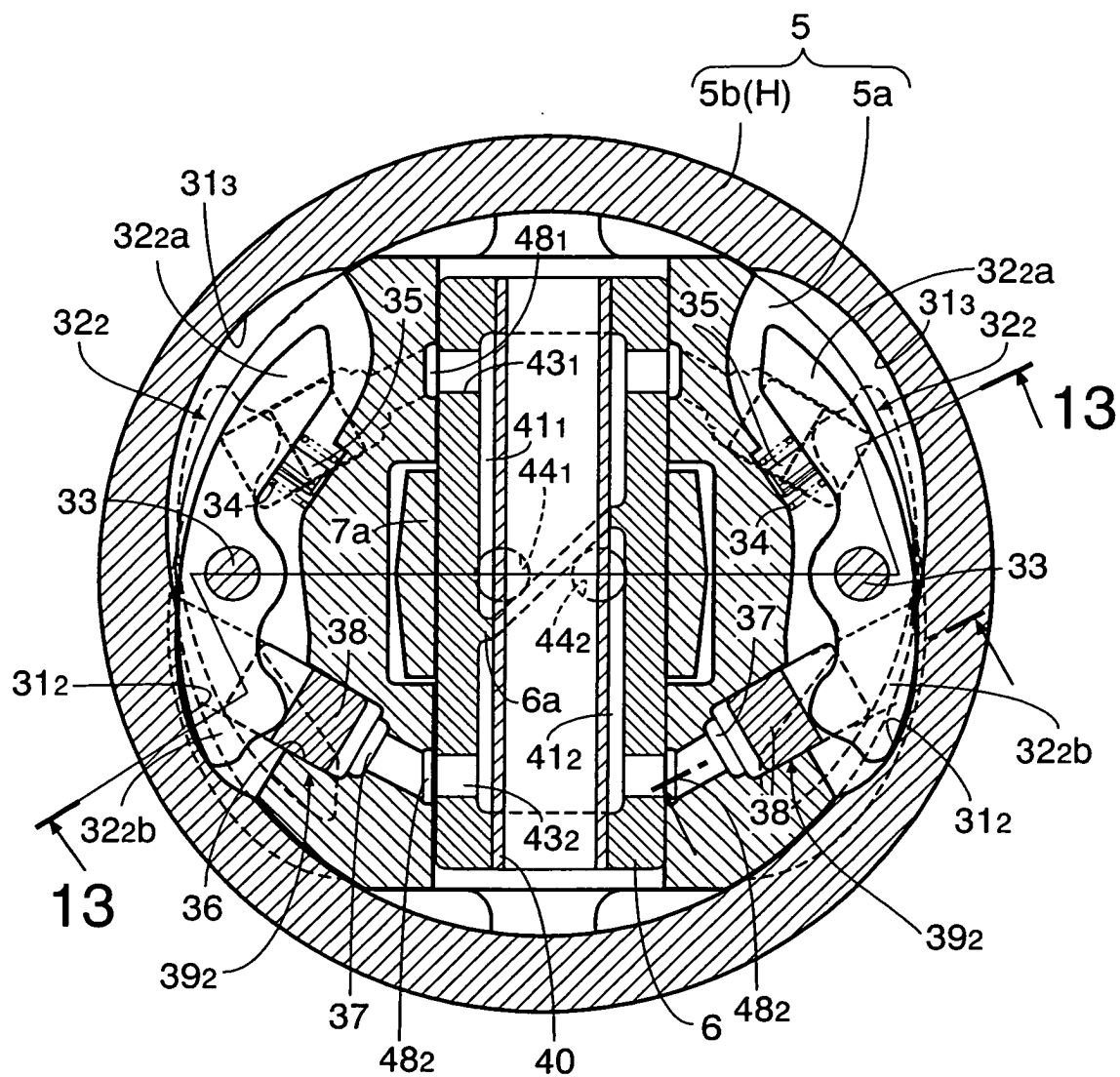
FIG.15 HIGH COMPRESSION RATIO STATE
