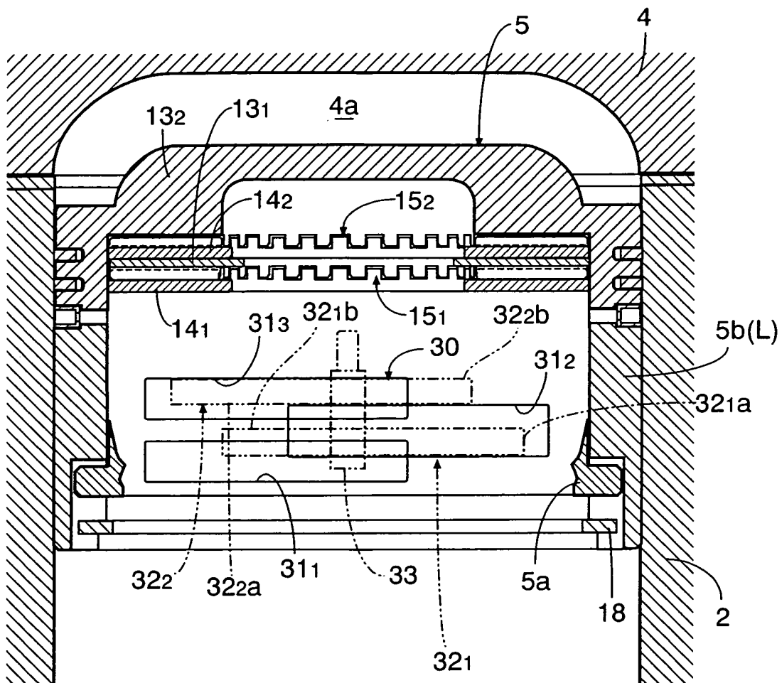
FIG.17 LOW COMPRESSION RATIO STATE
