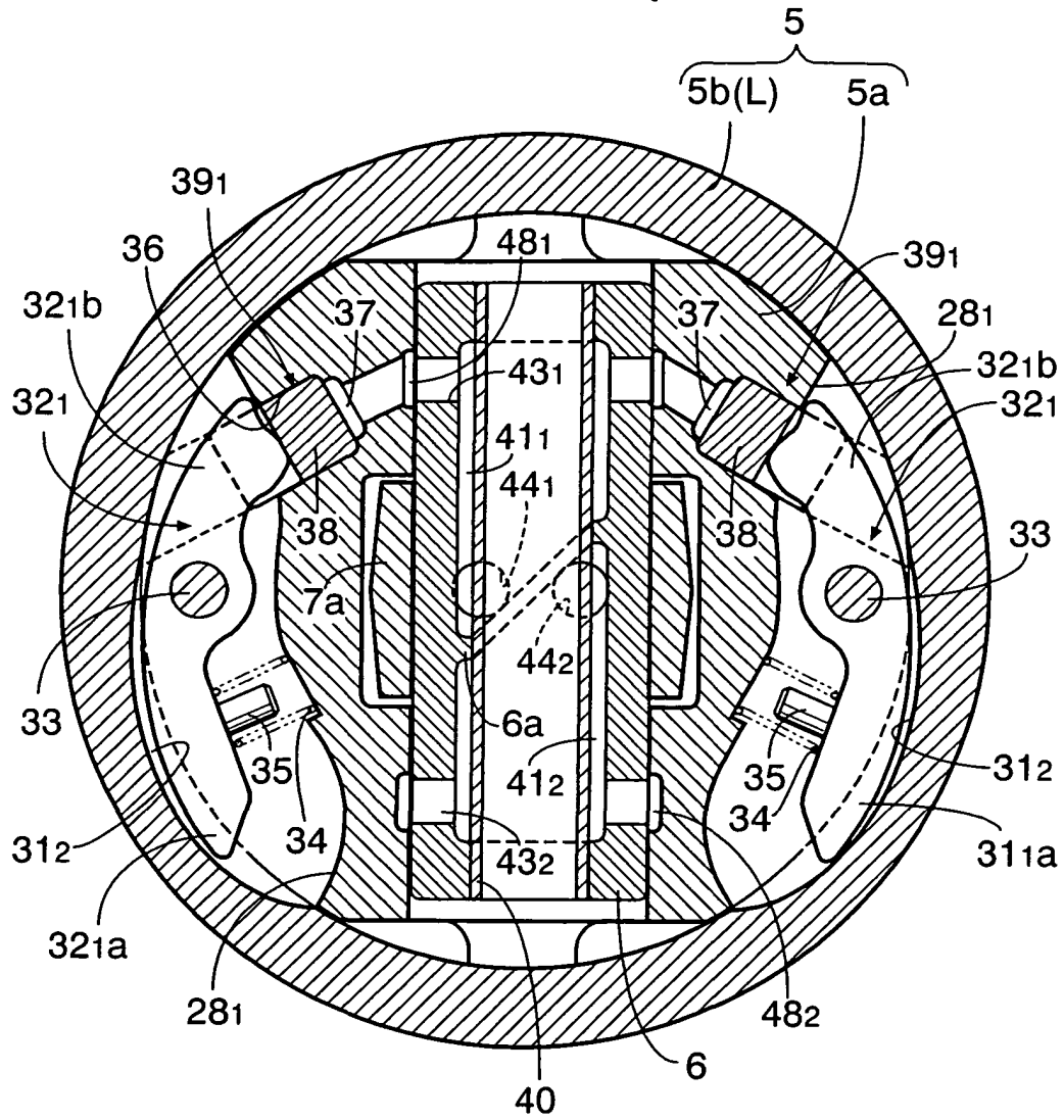
FIG.4 LOW COMPRESSION RATIO STATE
