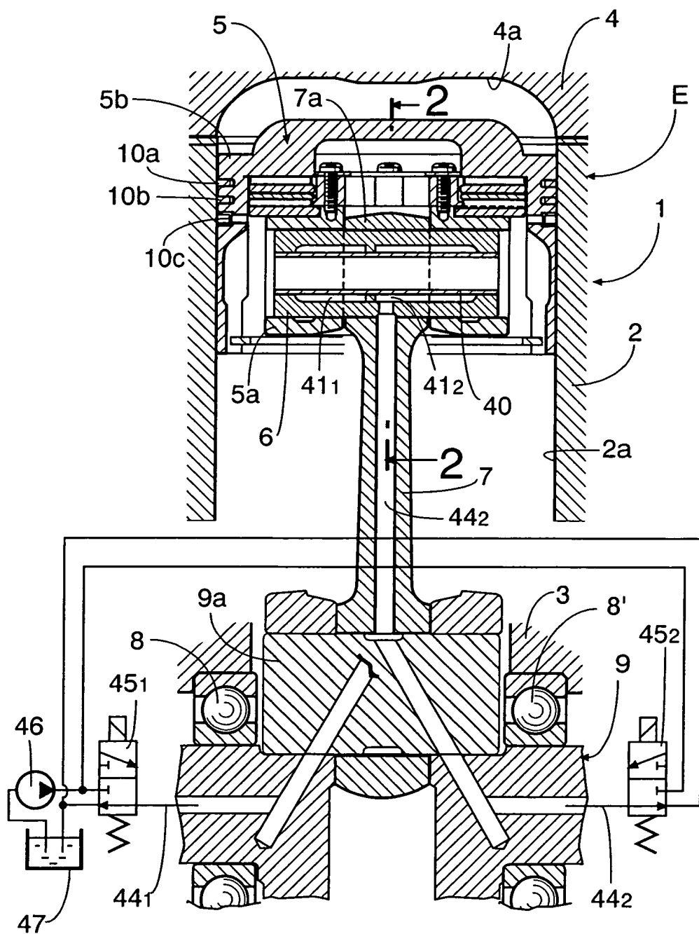
FIG.1 LOW COMPRESSION RATIO STATE
