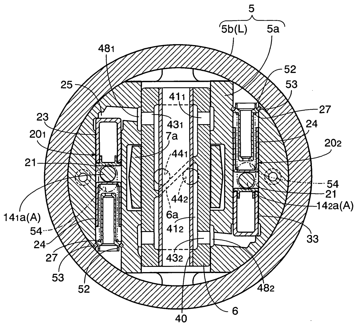
FIG.6 LOW COMPRESSION RATIO STATE
