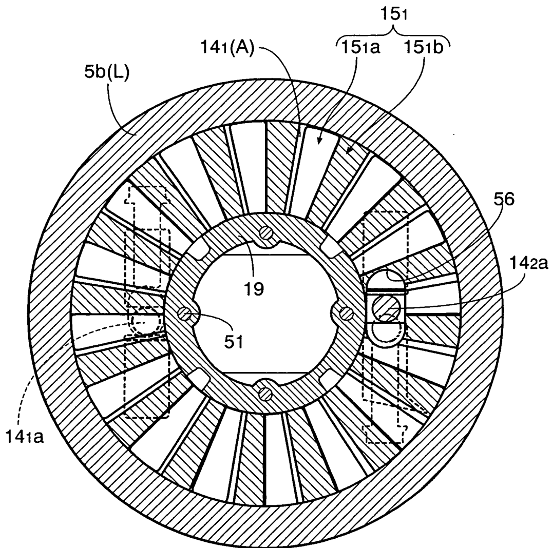
FIG.7 LOW COMPRESSION RATIO STATE
