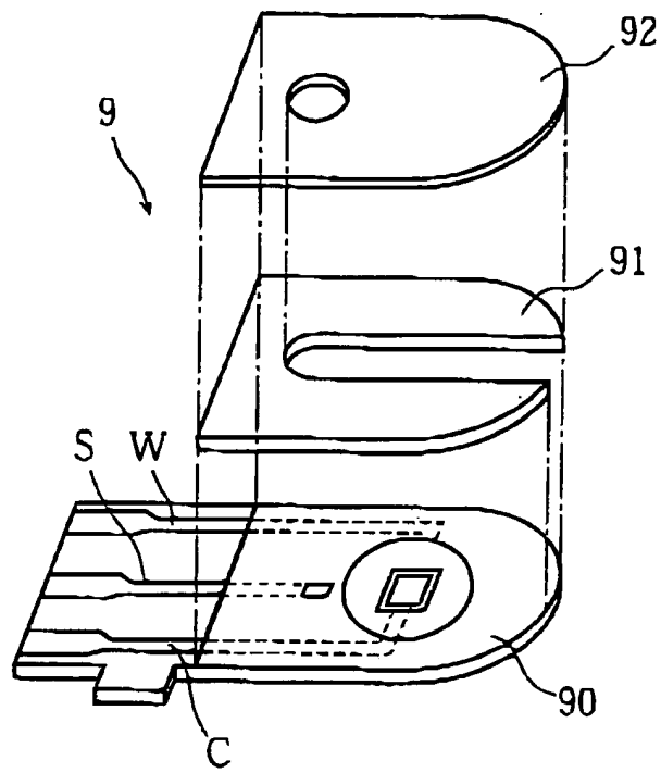
FIG.6 PRIOR ART
