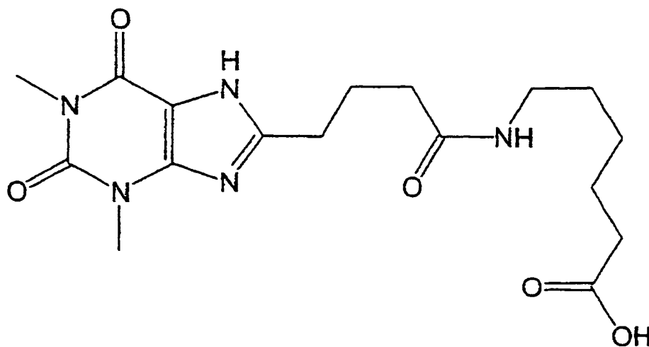
Theophylline · LC
