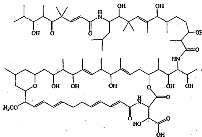
poecillastrin A (1)
