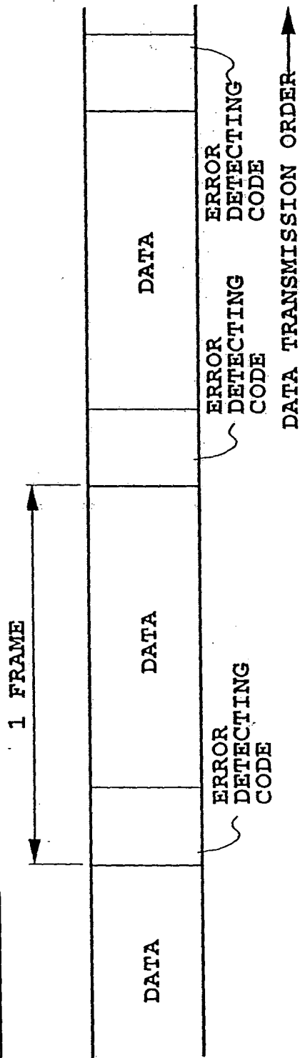
FIG.2A
