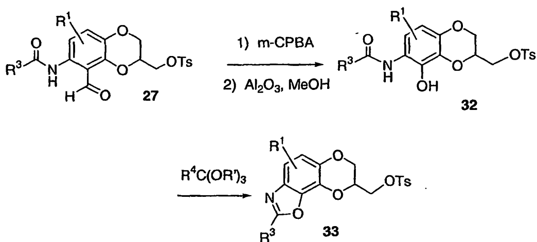
Scheme 11
