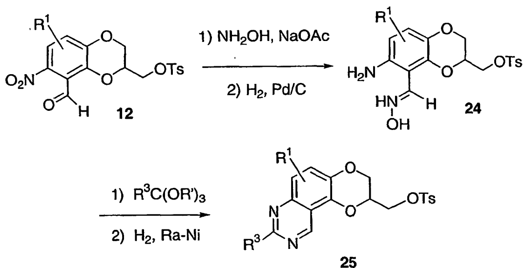
Scheme 8
