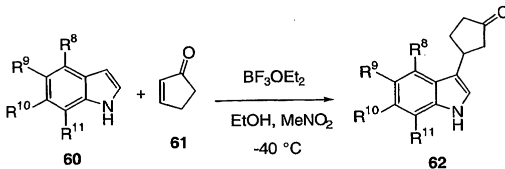
Scheme 20
