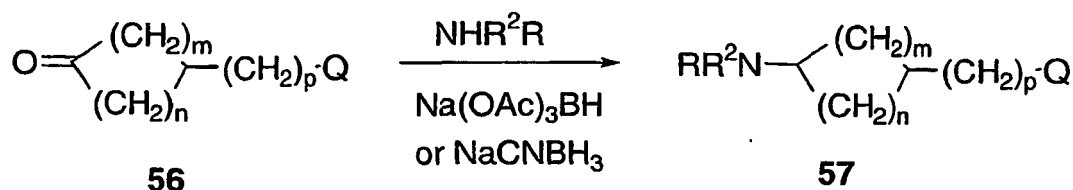
Scheme 18
