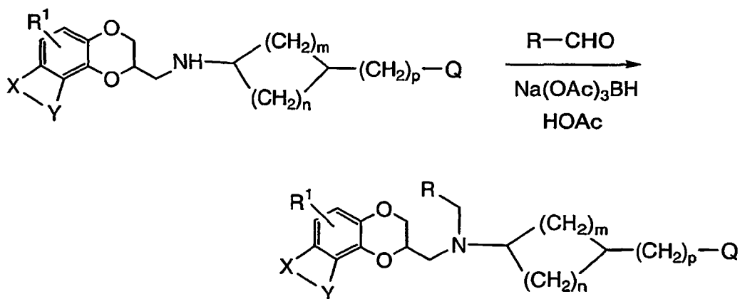
Scheme 3
