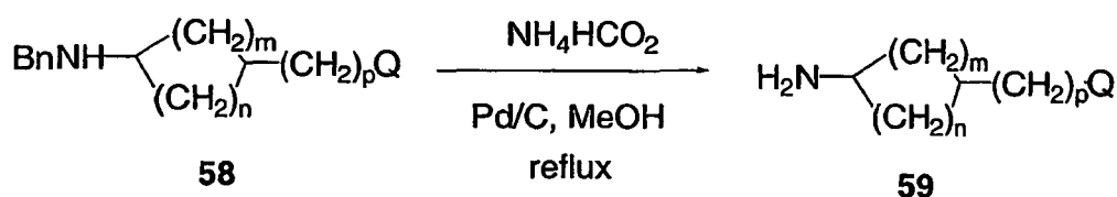
Scheme 19
