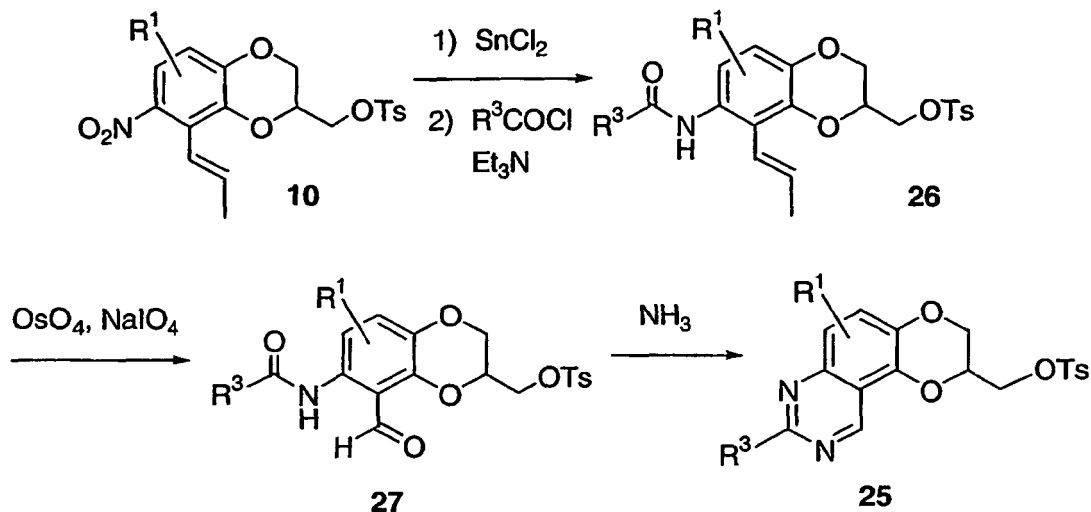
Scheme 9
