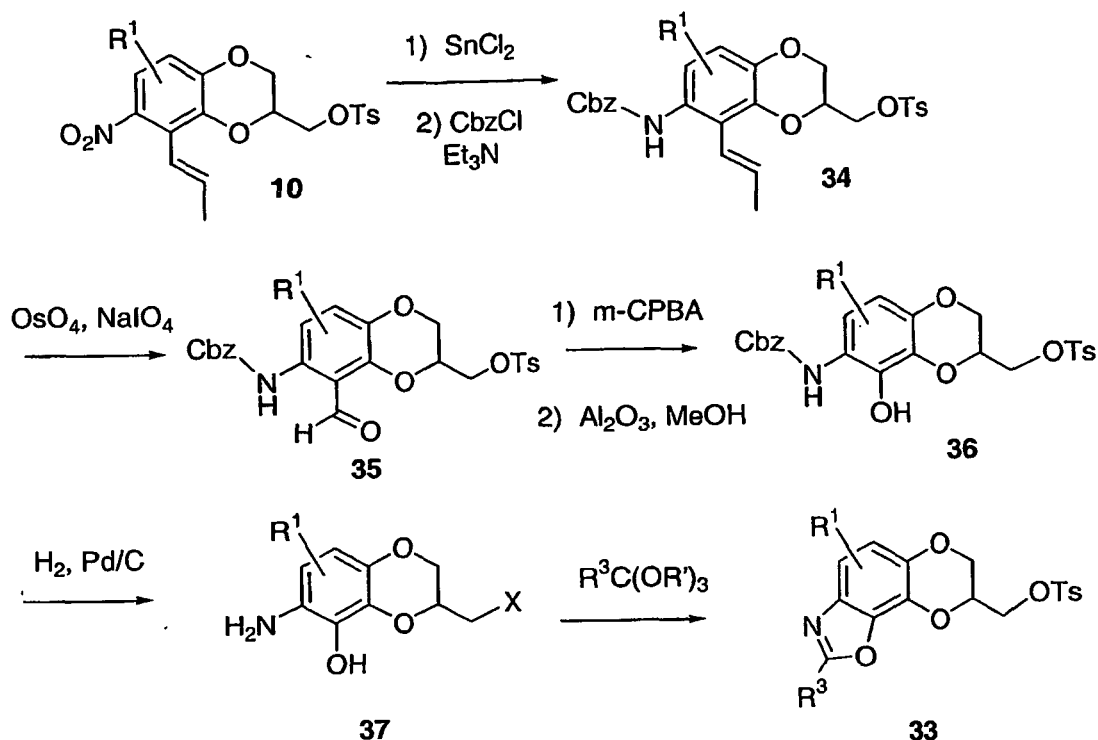
Scheme 12
