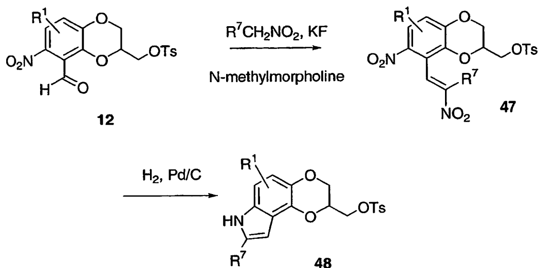
Scheme 16
