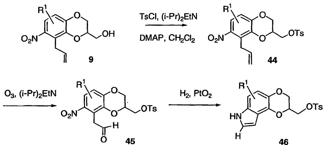
Scheme 15
