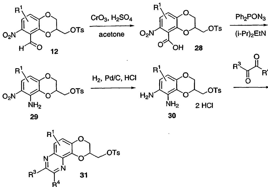
Scheme 10
