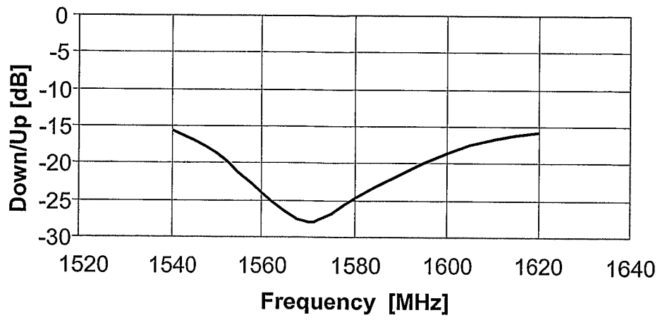
Down/Up Ratio in the Zenith Direction versus Frequency for a Receiving Antenna and Passive Antenna System
