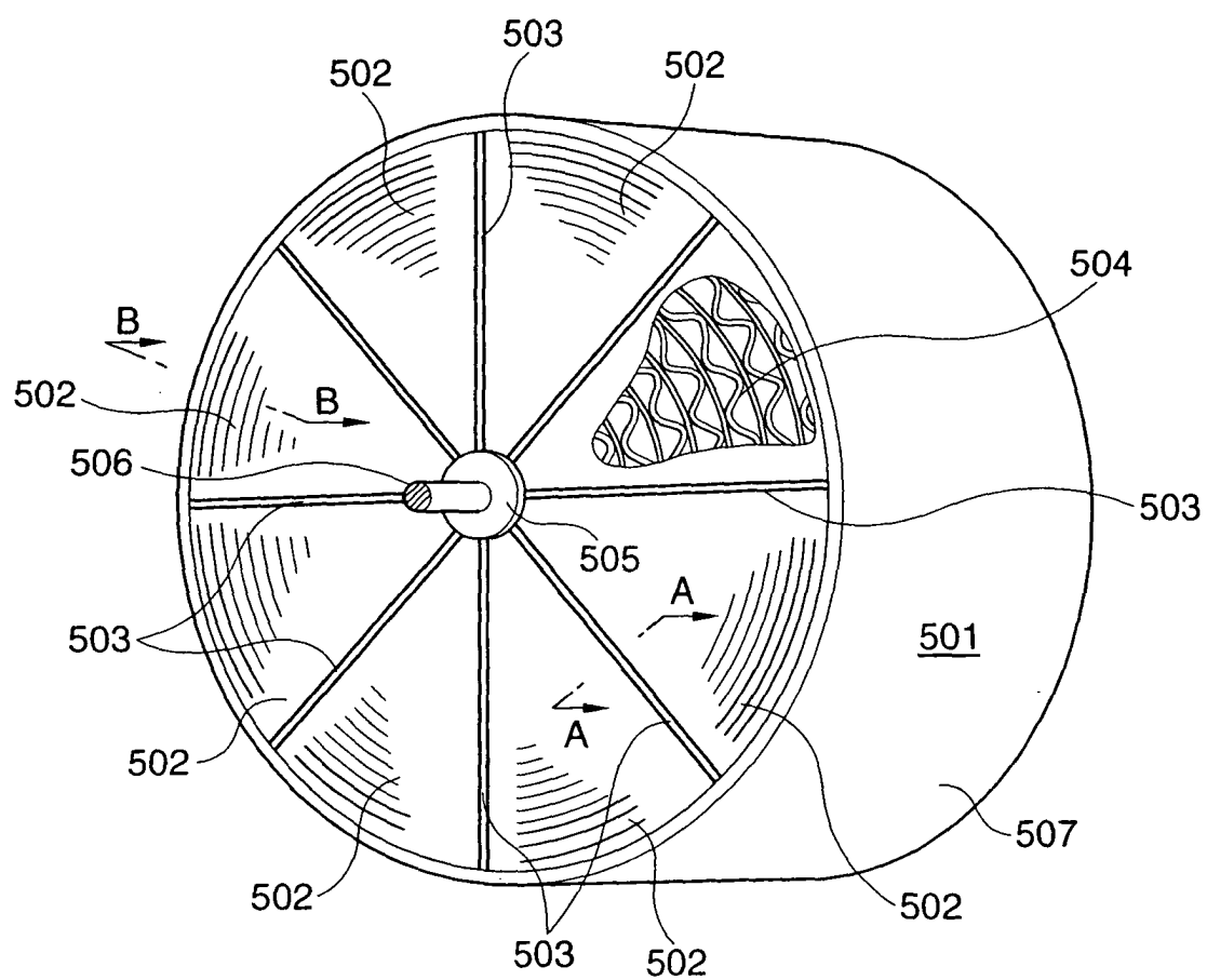
FIG. 12 PRIOR ART
