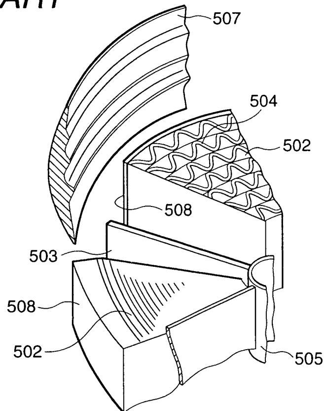
FIG. 14 PRIOR ART
