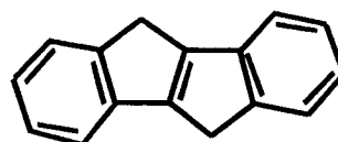
5,10-dihydroindeno[2,1-a]indene
