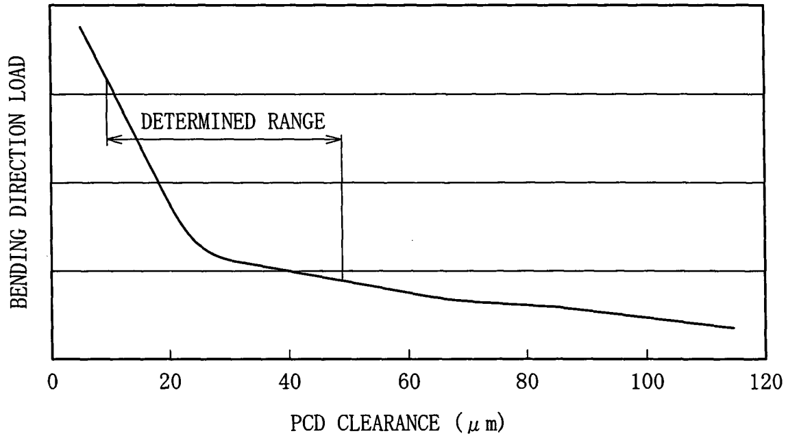
PCD CLEARANCE SENSITIVITY CHART
