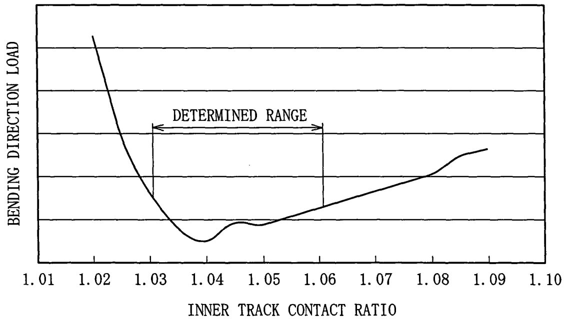
INNER-RING TRACK CONTACT RATIO SENSITIVITY CHART
