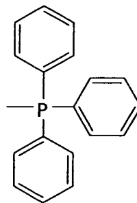
triphenylphosphine
