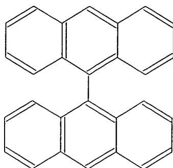
9, 9' -bianthryl
