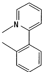
cyclometalate
