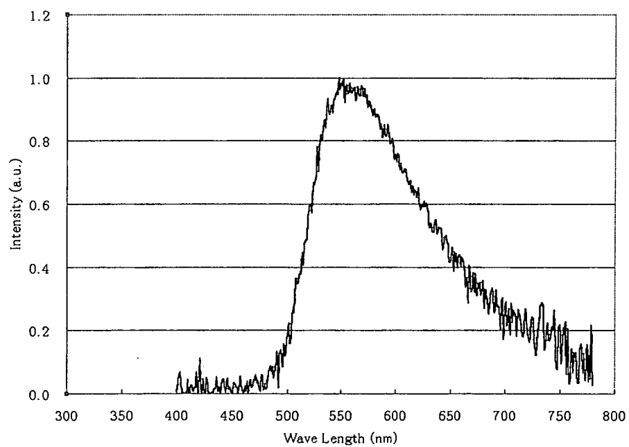
Pt(bcp)(dce) PL spectrum
