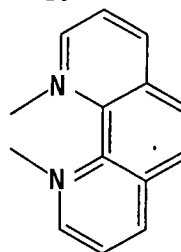
1,10-phenanthroline
