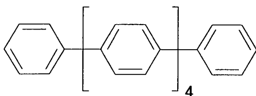
p-sexiphenyl
