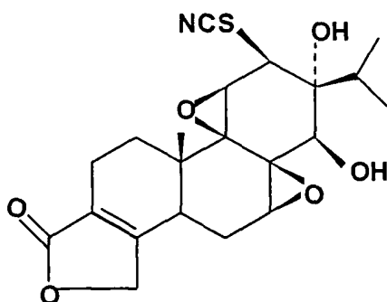
12- \beta -thiocyano-13- \alpha -hydroxy triptolide (T-SCN)
