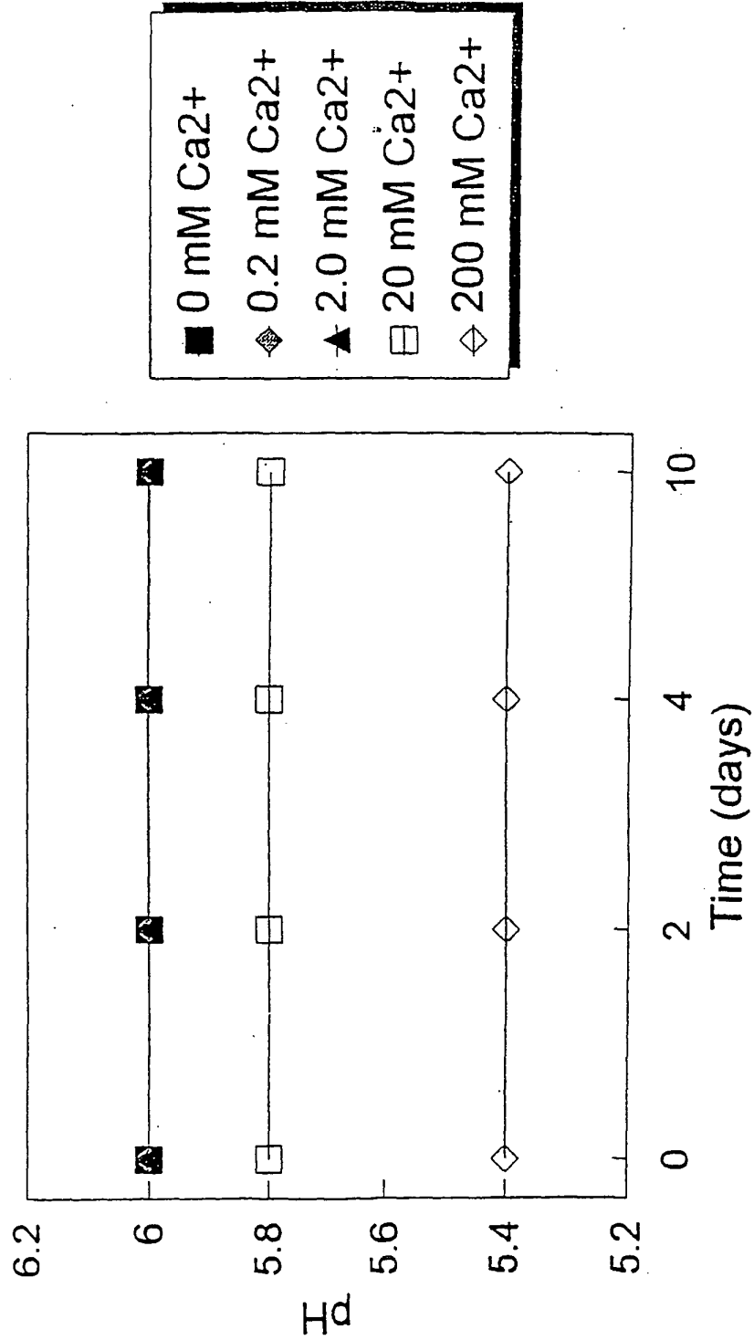
Figure 2. The Effect of Carbon Dioxide and Calcium Ion on the pH of a Calcium Carbonate Slurry
