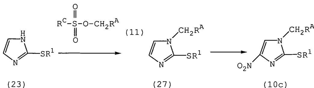
Reaction scheme-9
