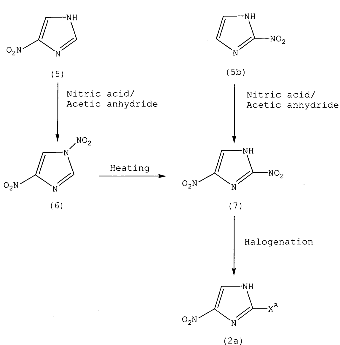
Reaction scheme-1
