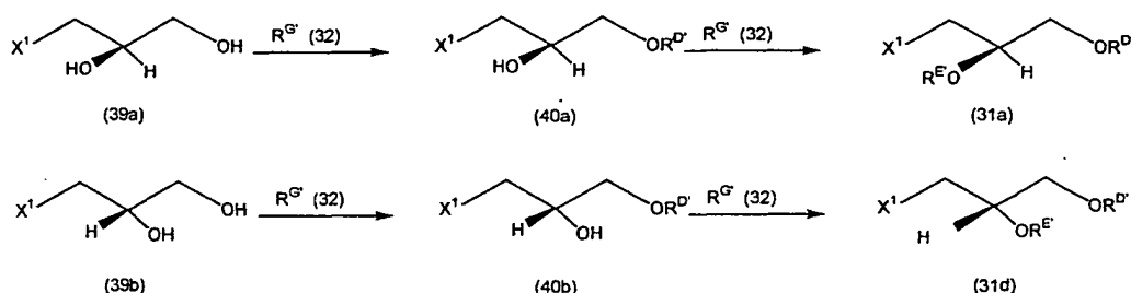
Reaction scheme-14
