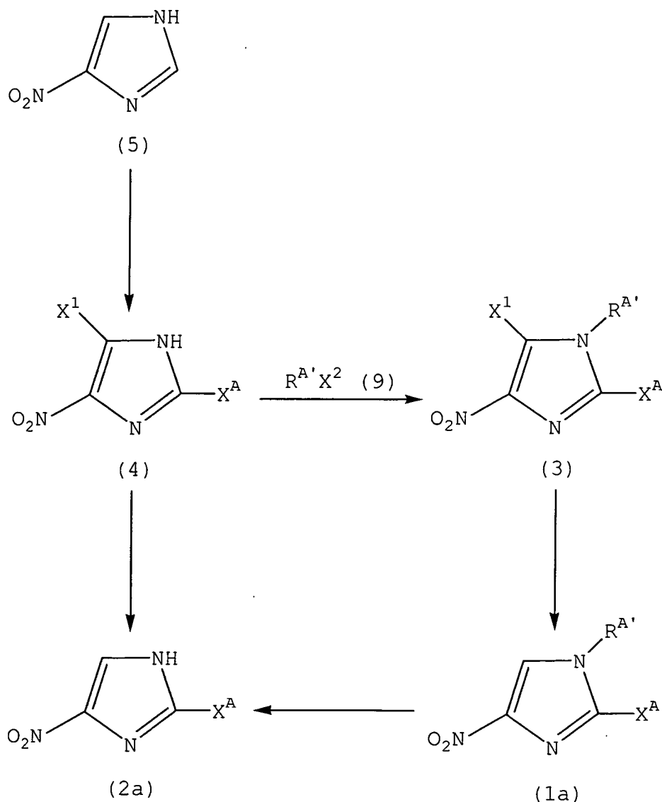
Reaction scheme-3
