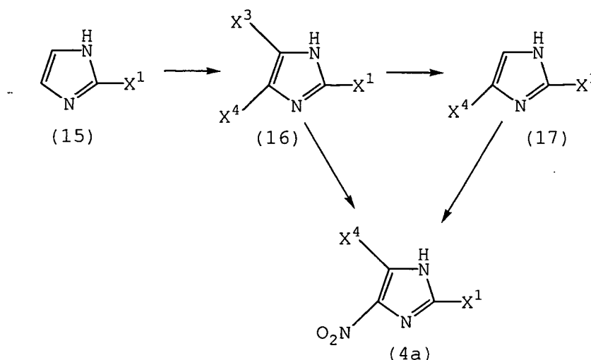
Reaction scheme-6
