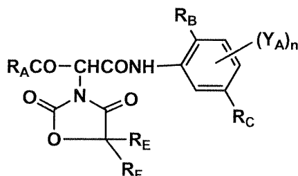
formula (3)
