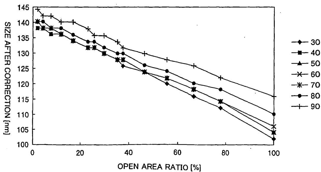
RELATION BETWEEN OPEN AREA RATIO AND SIZE AFTER CORRECTION WHEN \beta F VALUE IS VARIED
