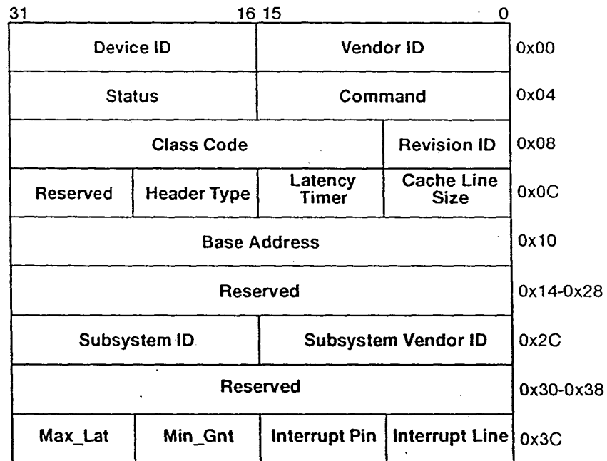
Figure 1.1 the coprocessor PCI Configuration Space Layout
