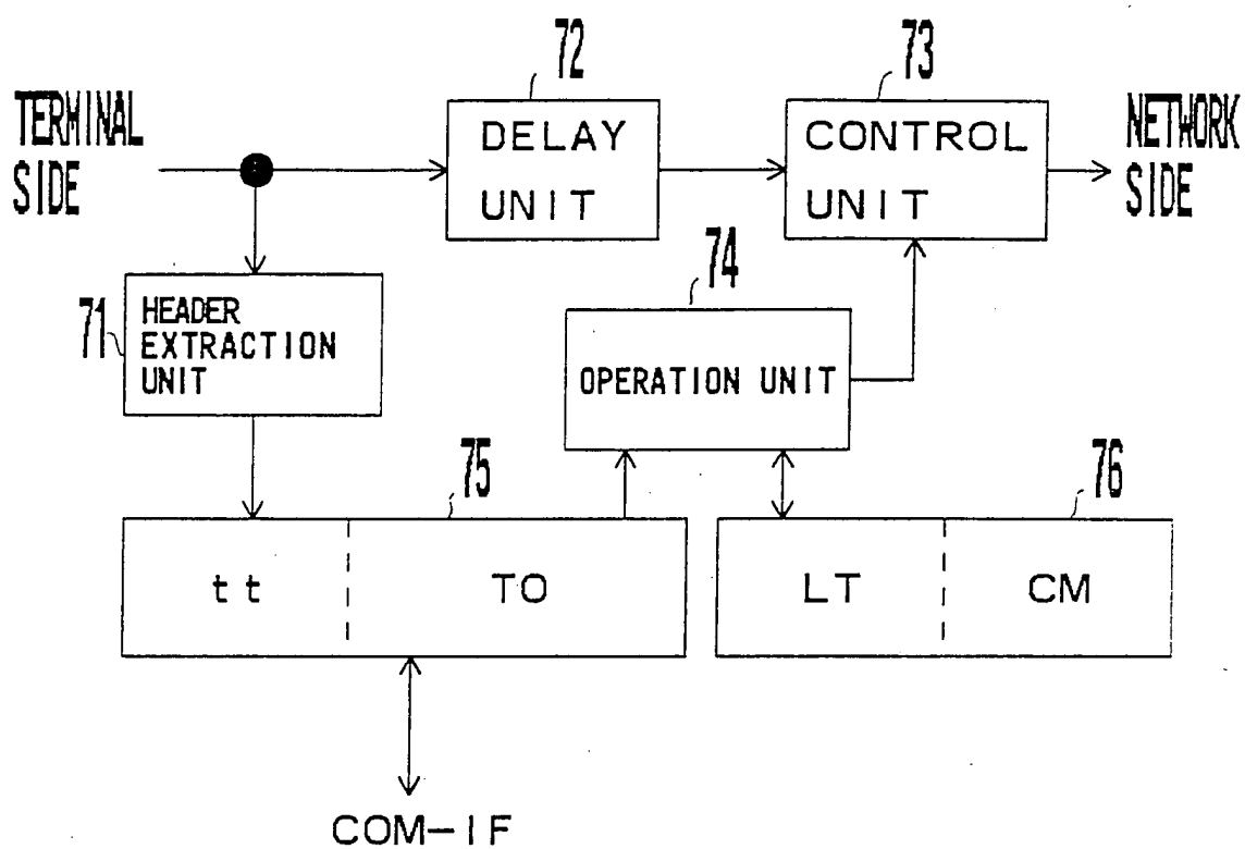
FIG. 7 PRIOR ART
