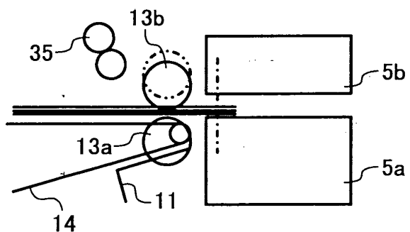
FIG. 9C STAPLER MOVEMENT
