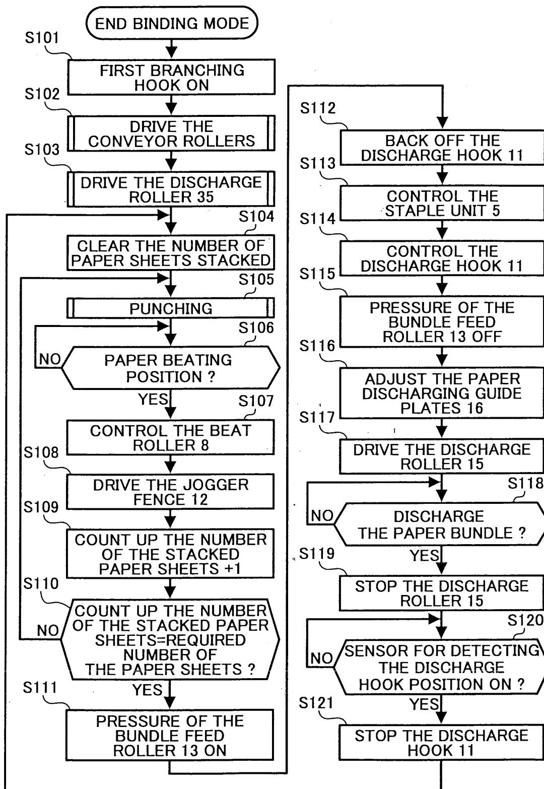
FIG. 19 END BINDING MODE
