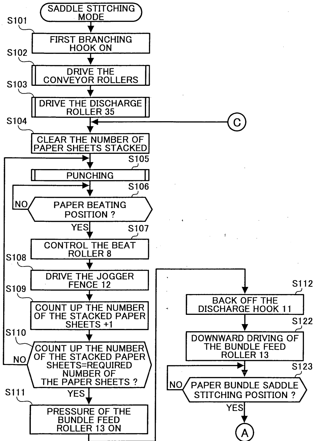
FIG. 20A SADDLE STITCHING MODE
