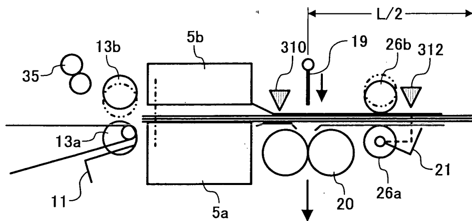
FIG. 10D FOLDING
