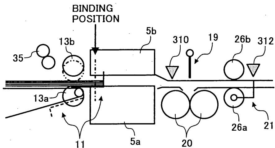
FIG. 10A ADJUSTMENT
