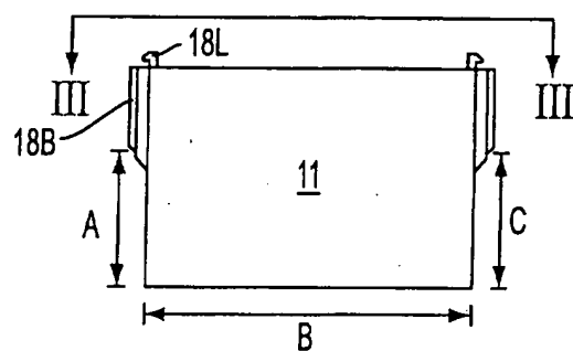
FIG. 2 (PRIOR ART)
