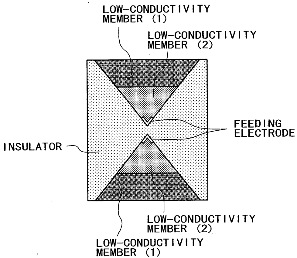
CROSS-SECTIONAL VIEW
