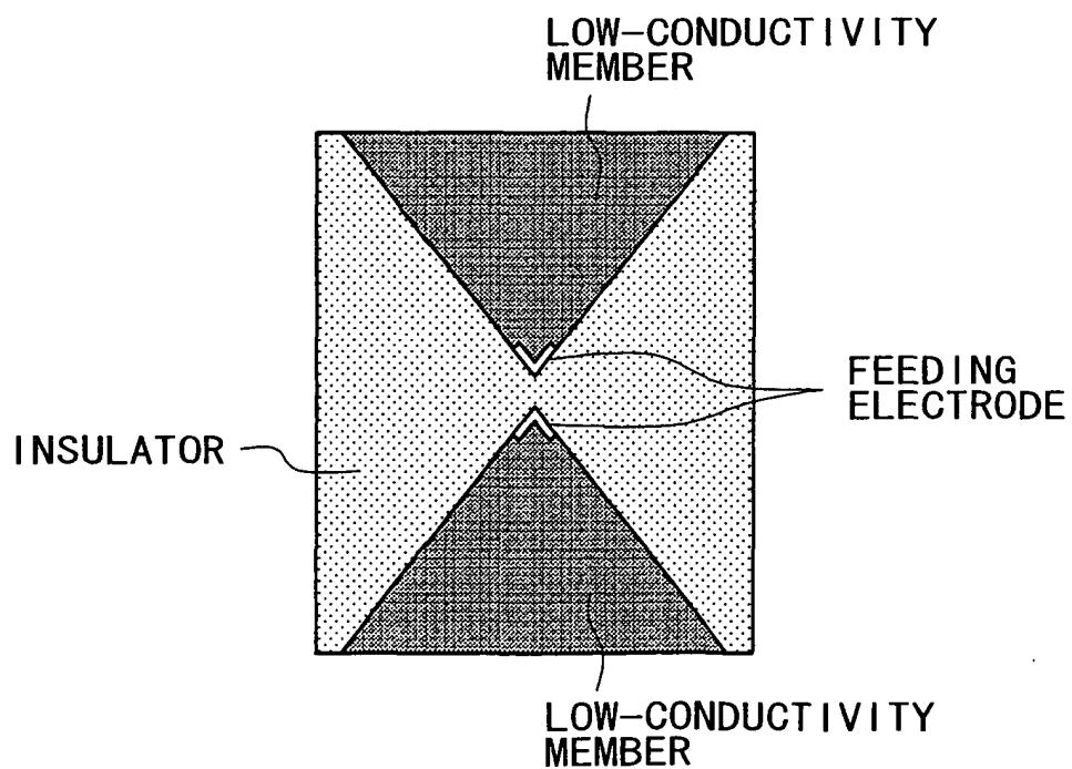
CROSS-SECTIONAL VIEW
