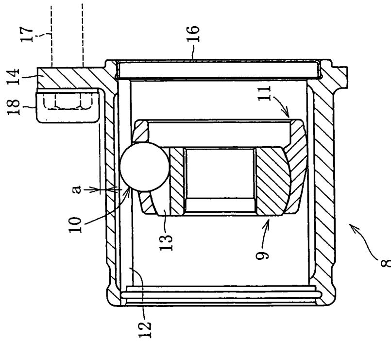
FIG. 23a Prior Art
