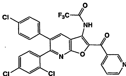
N'-[5-(4-Chlorophenyl)-6-(2,4-dichlorophenyl)-2-(pyridin-3-ylcarbonyl)furo[2,3-b]pyridin-3-yl]-2,2,2-trifluoroacetamide
