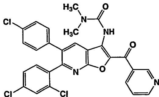
N'-[5-(4-Chlorophenyl)-6-(2,4-dichlorophenyl)-2-(pyridin-3-ylcarbonyl)furo[2,3-b]pyridin-3-yl]-N,N-dimethylurea
