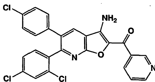
[3-Amino-5-(4-chlorophenyl)-6-(2,4-dichlorophenyl)furo[2,3-b]pyridin-2-yl](pyridin-3-yl)methanone
