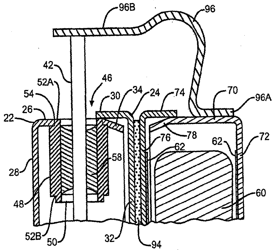
FIG. 3 Prior Art
